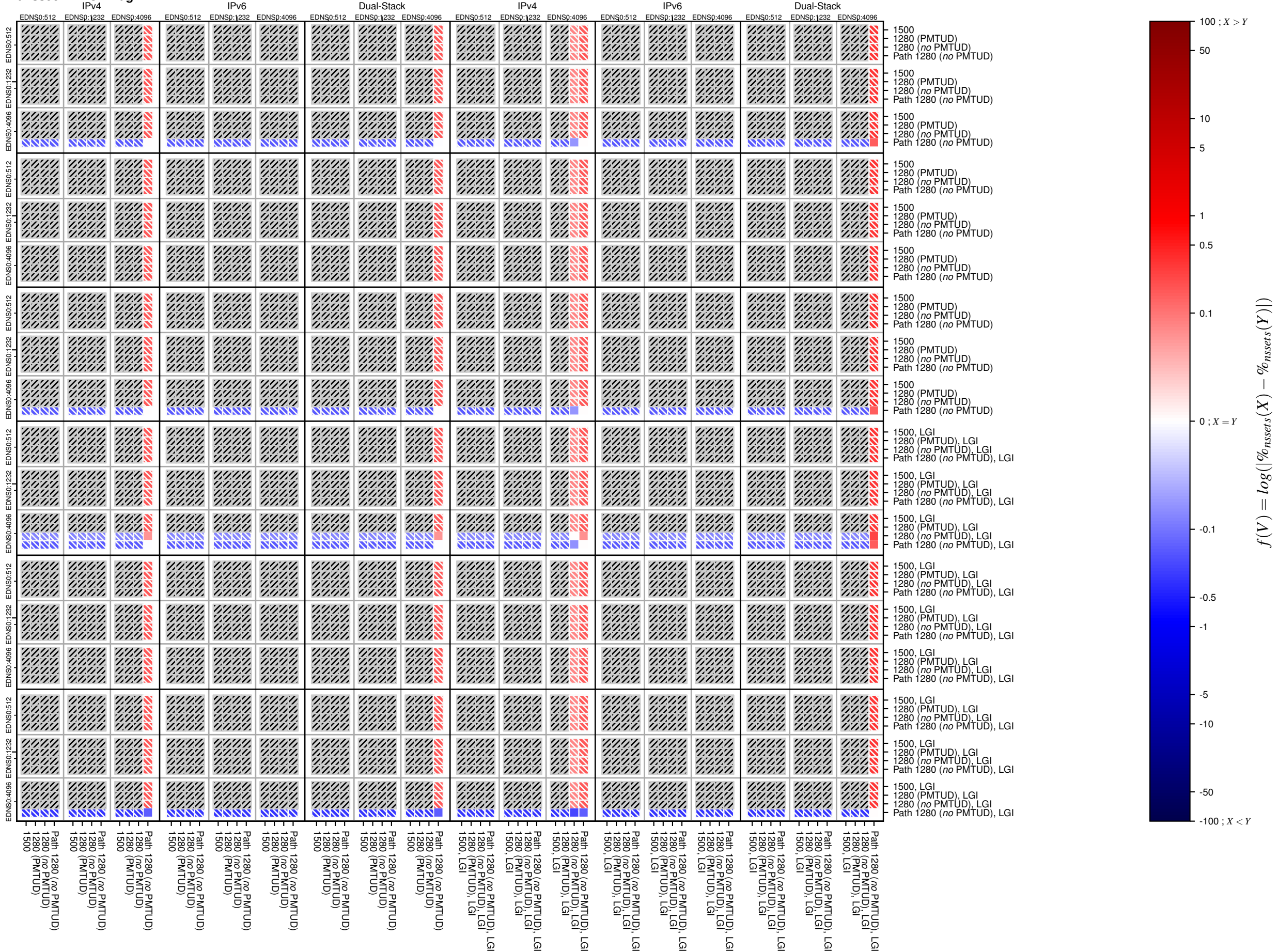
dnssec-v4-TCP_frag
