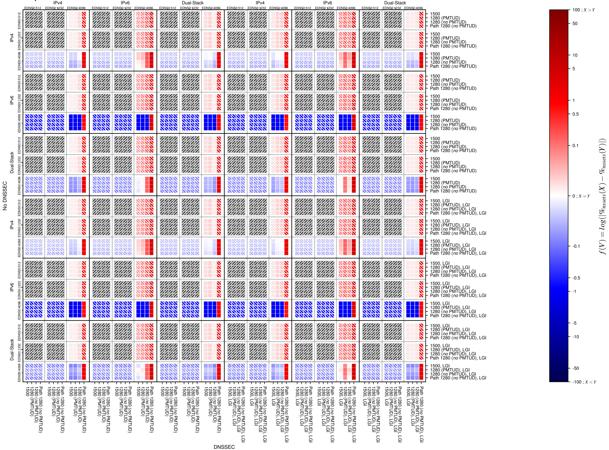
comp_dnssec-both-UDP_client_edns_fallback
