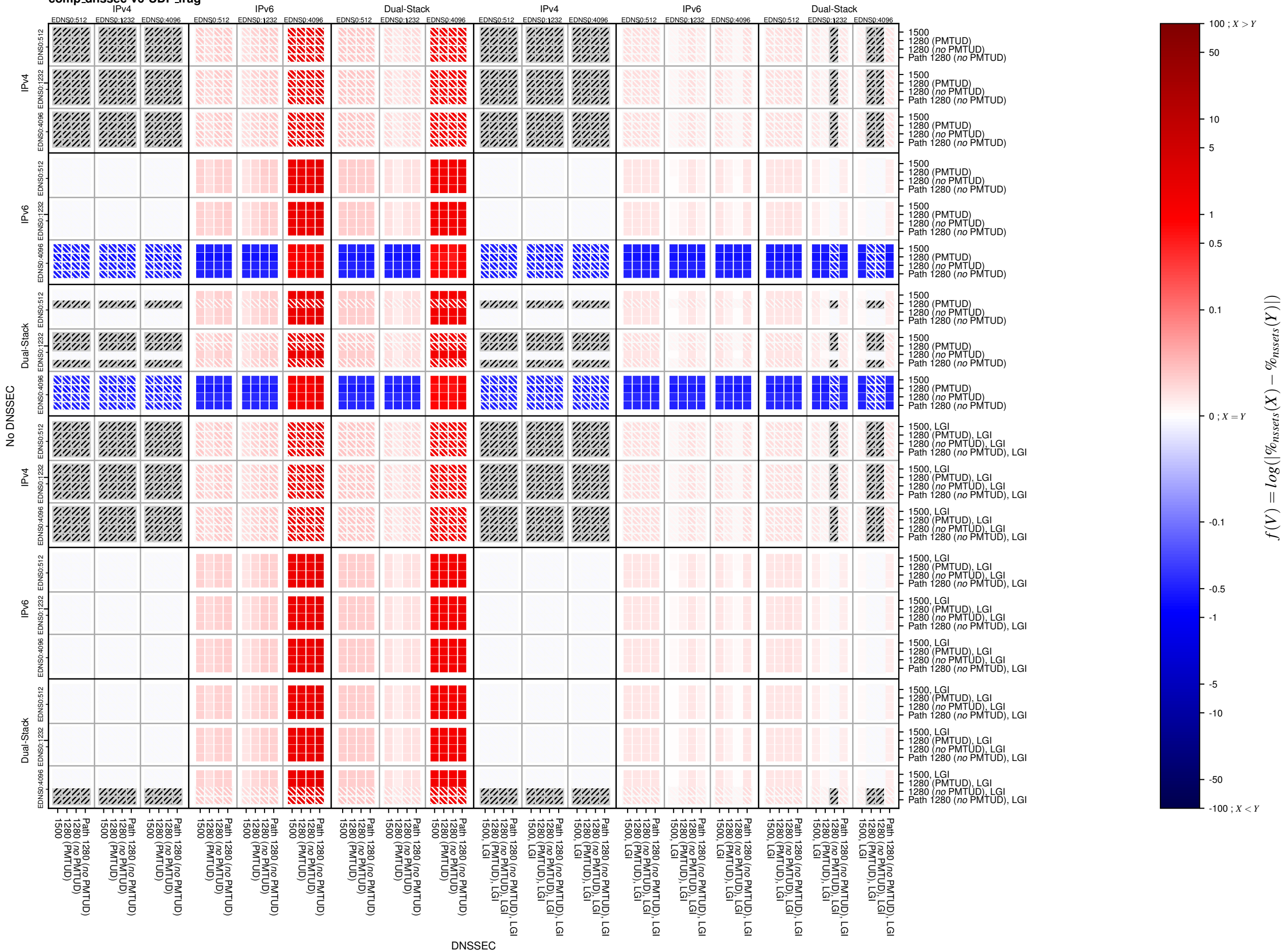
comp_dnsssec-v6-UDP_frag
