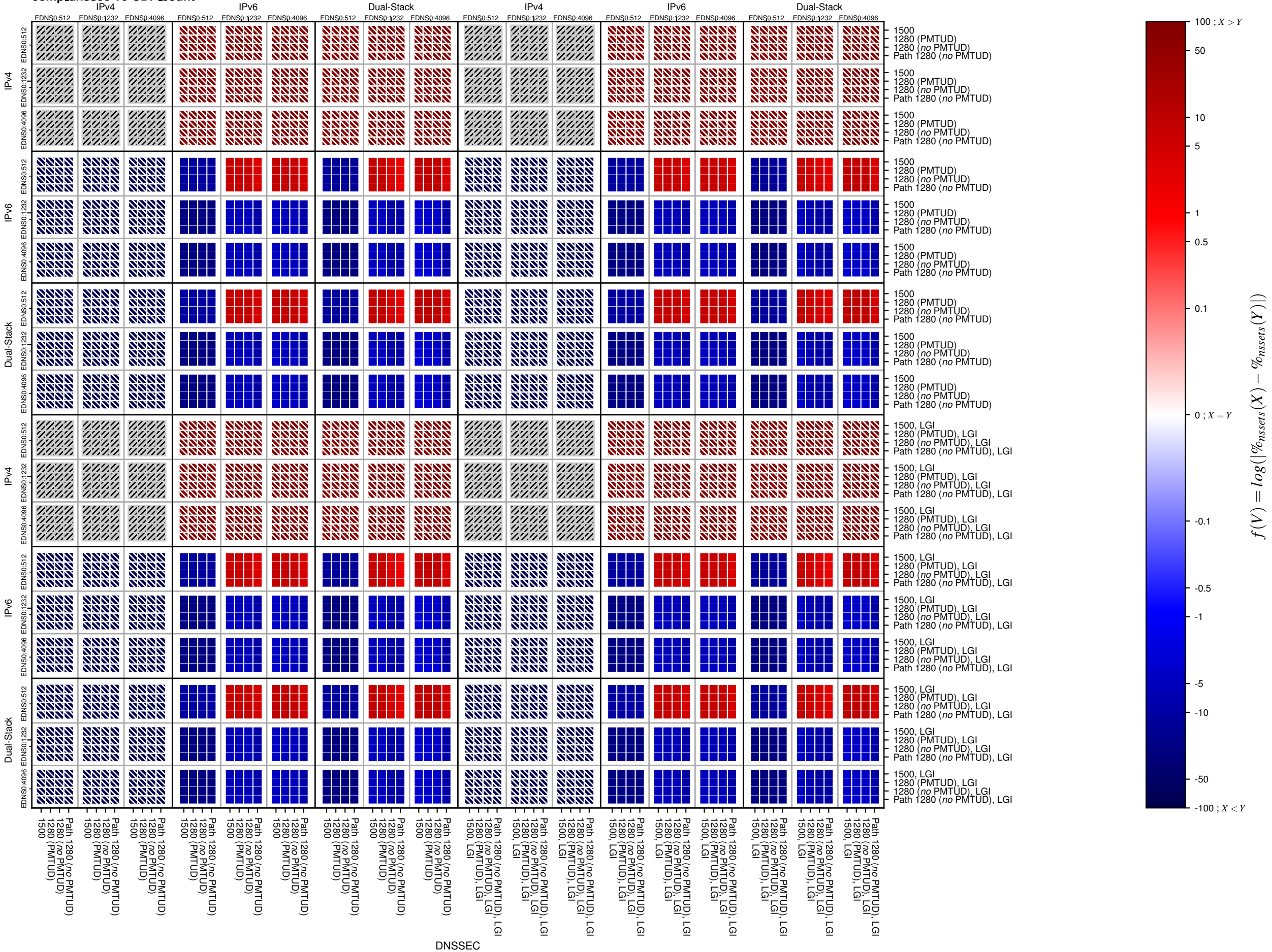
comp_dnssec-v6-UDP_count
