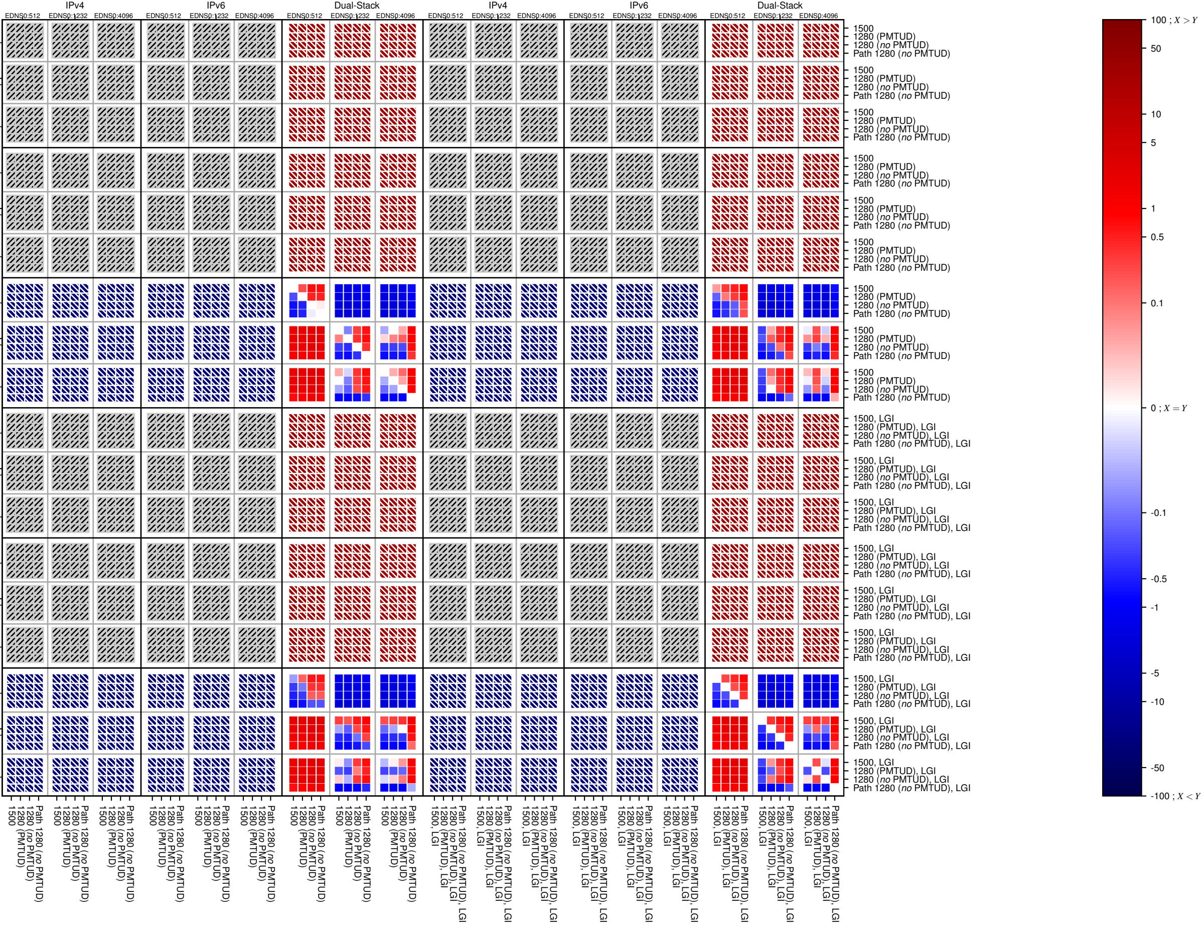
dnssec-v6-UDP_TCP_afi_count
