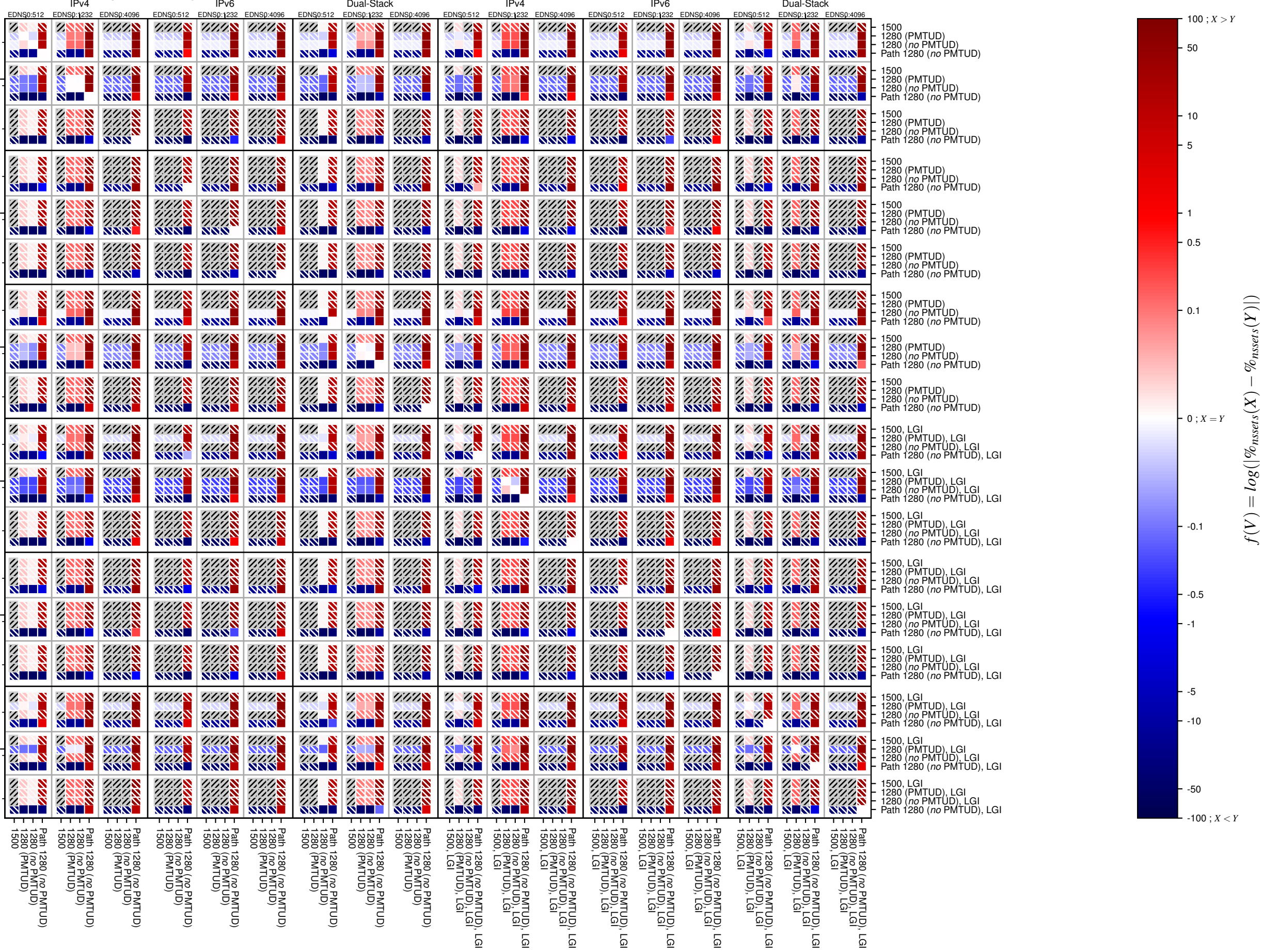
dnssec-both-TCP_packet_too_big
