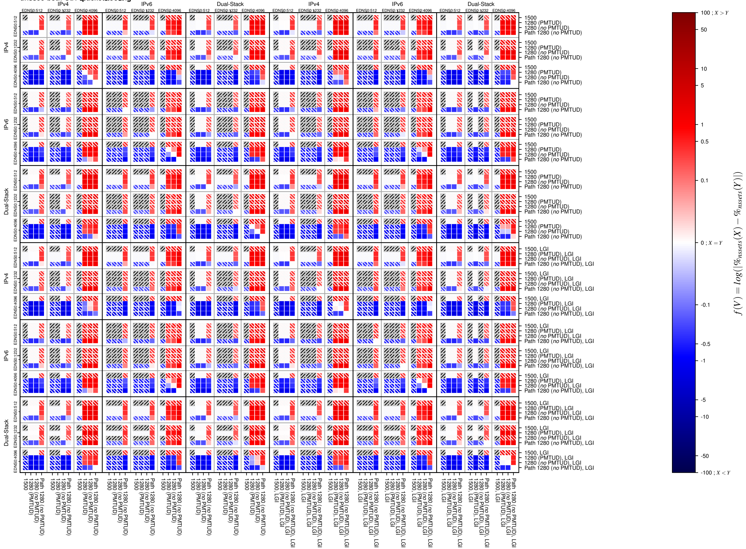
dnssec-both-UDP_packet_too_big
