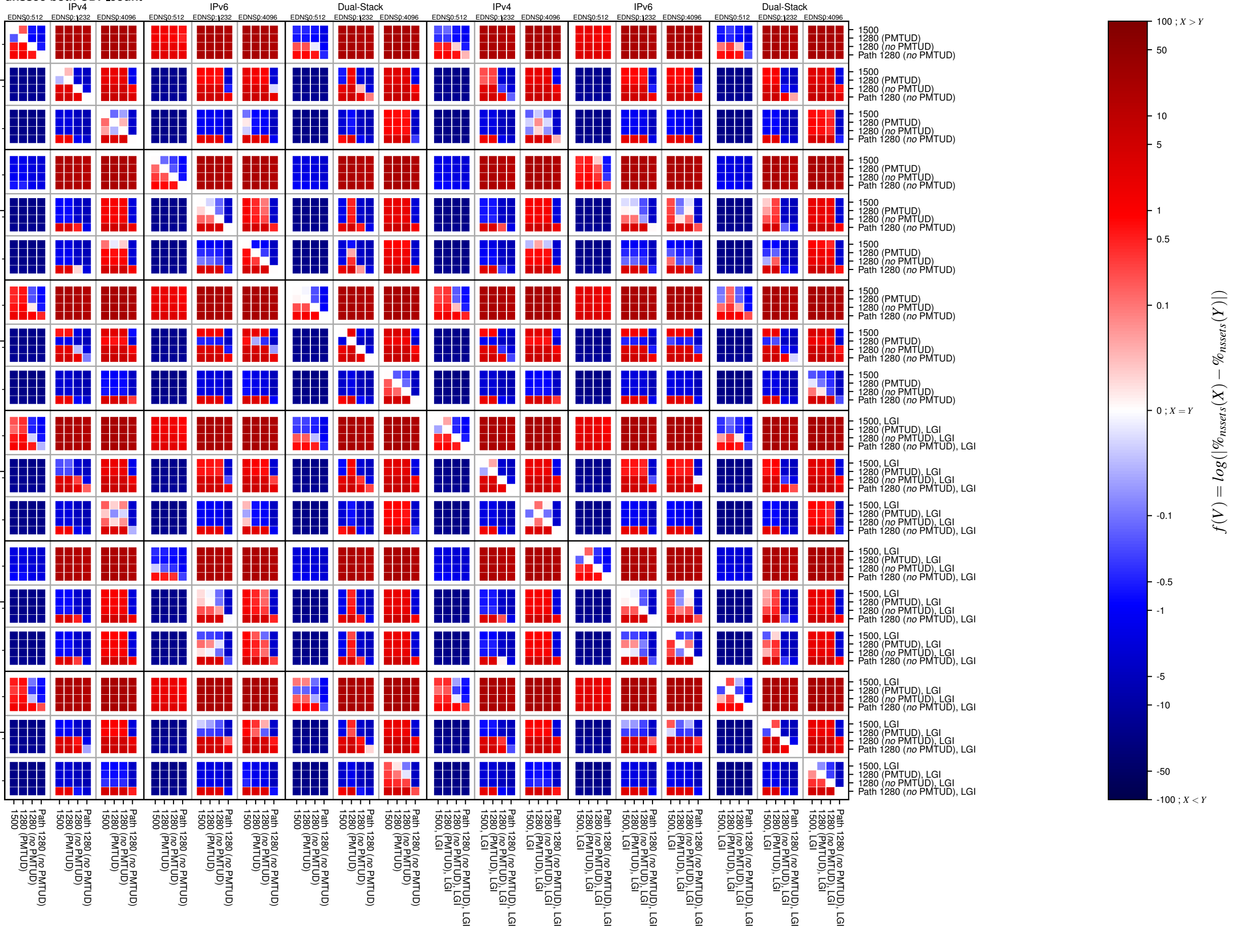
dnssec-both-UDP_count
