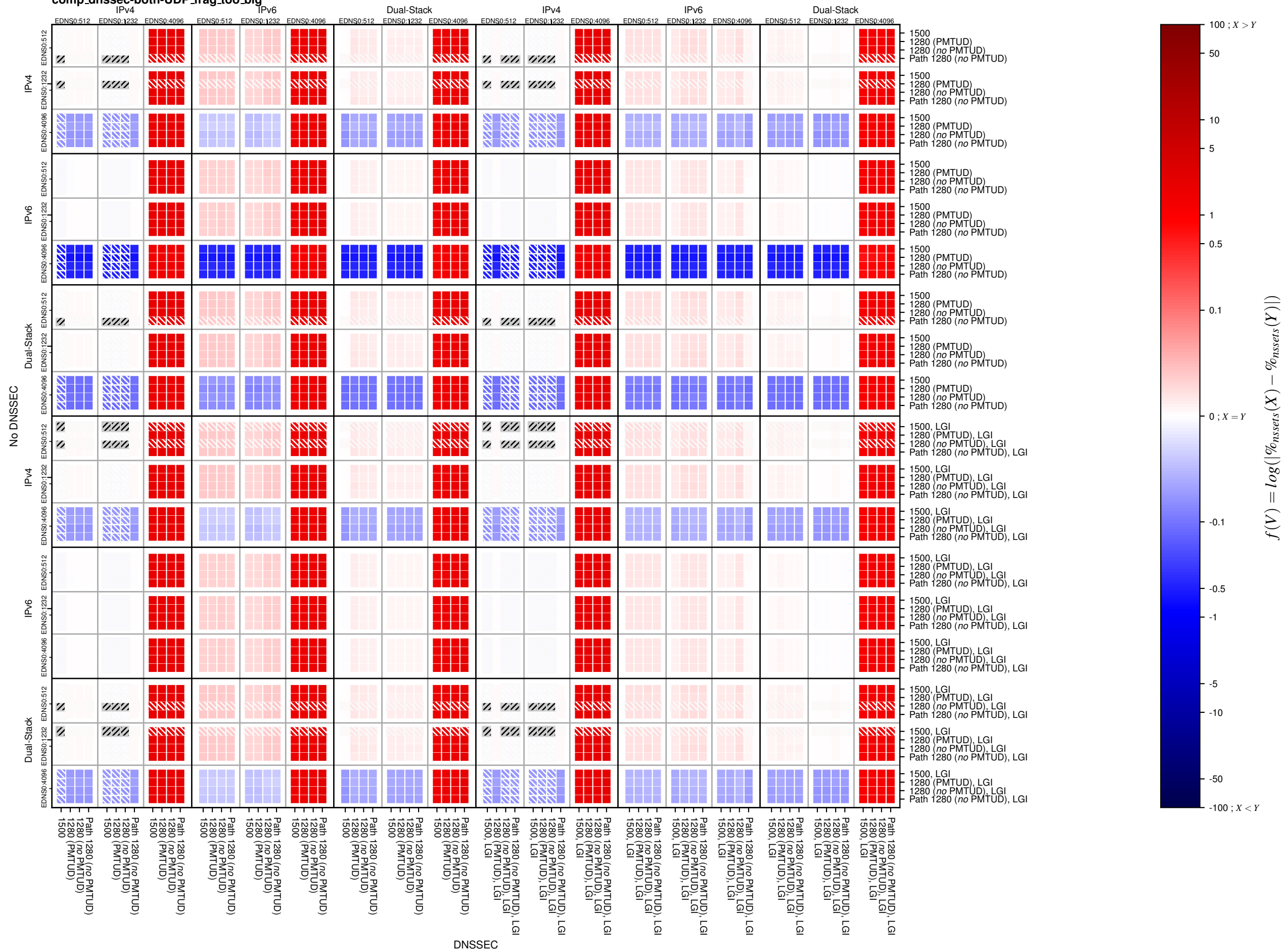
comp_dnsssec-both-UDP_frag_too_big
