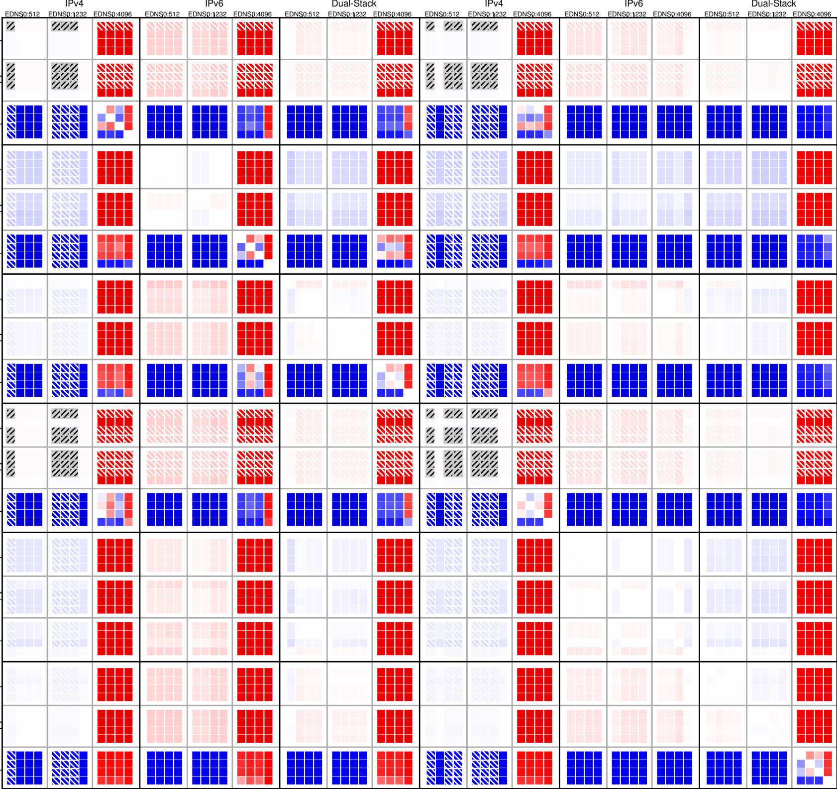
dnssec-both-UDP_frag_too_big
