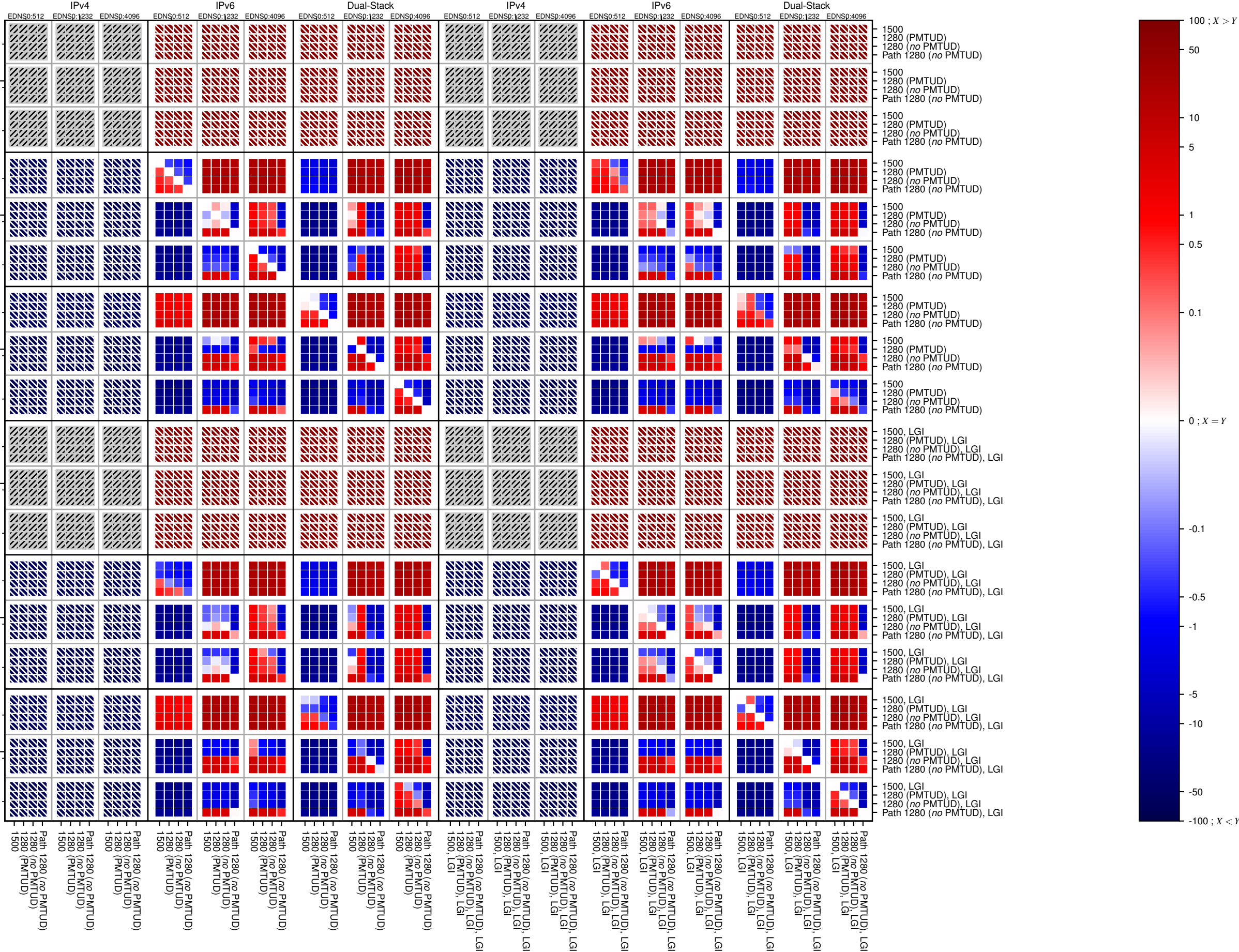
dnssec-v6-UDP_count
