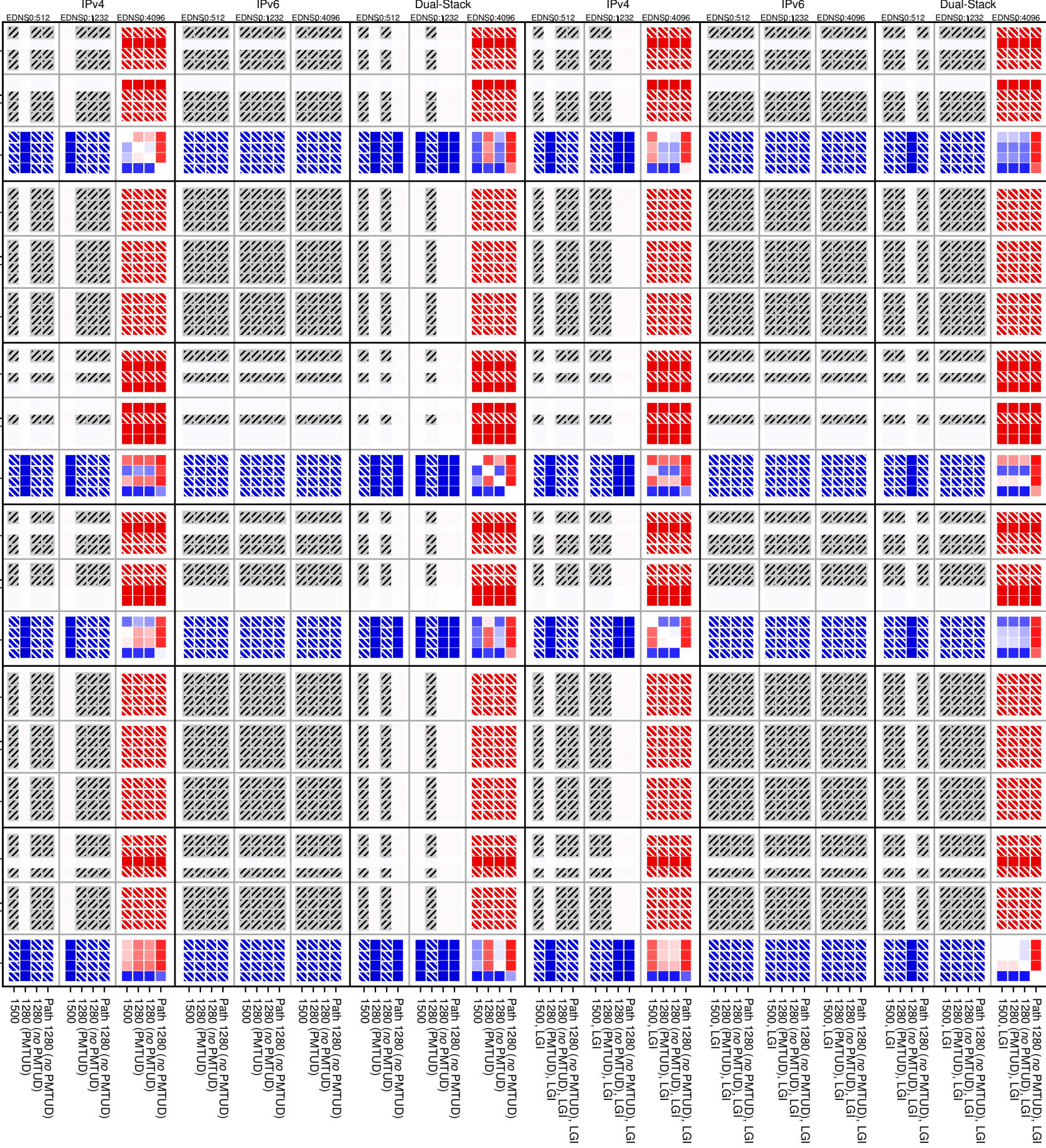
dnssec-v4-UDP_frag.too.big
