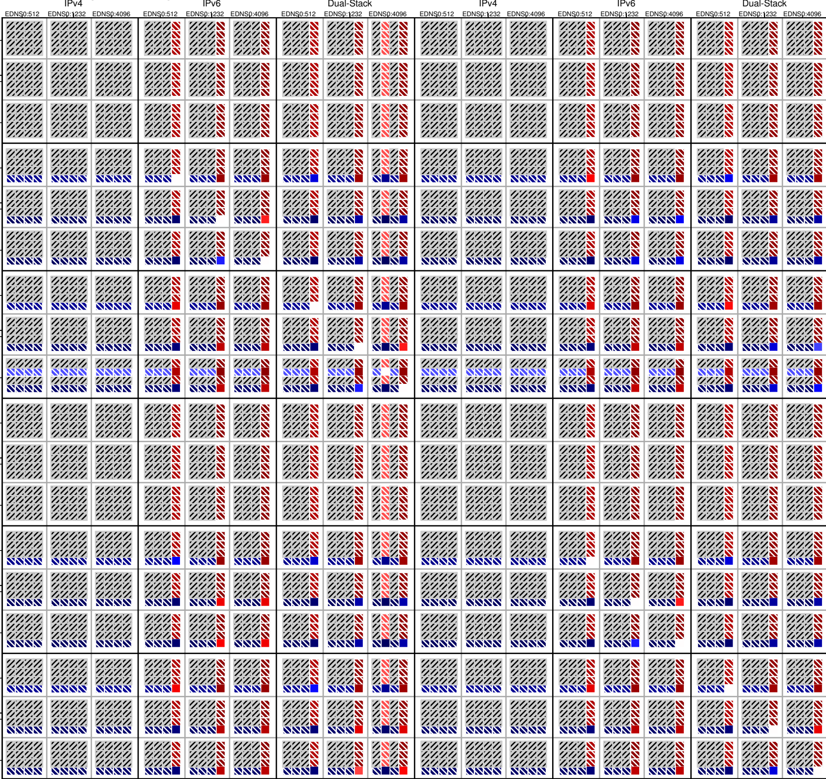
dnssec-v6-TCP_packet_too_big
