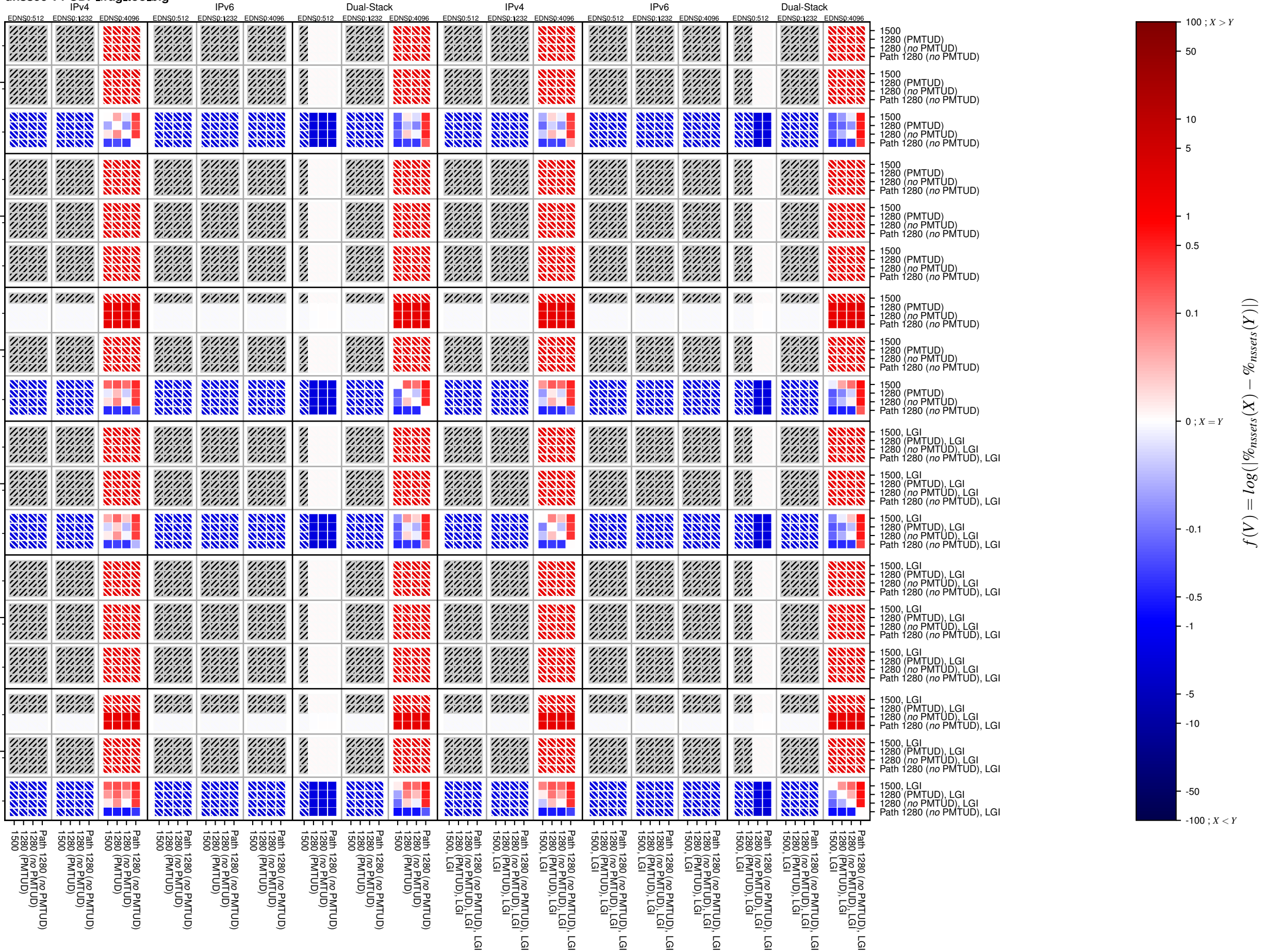
dnssec-v4-UDP_frag_too_big
