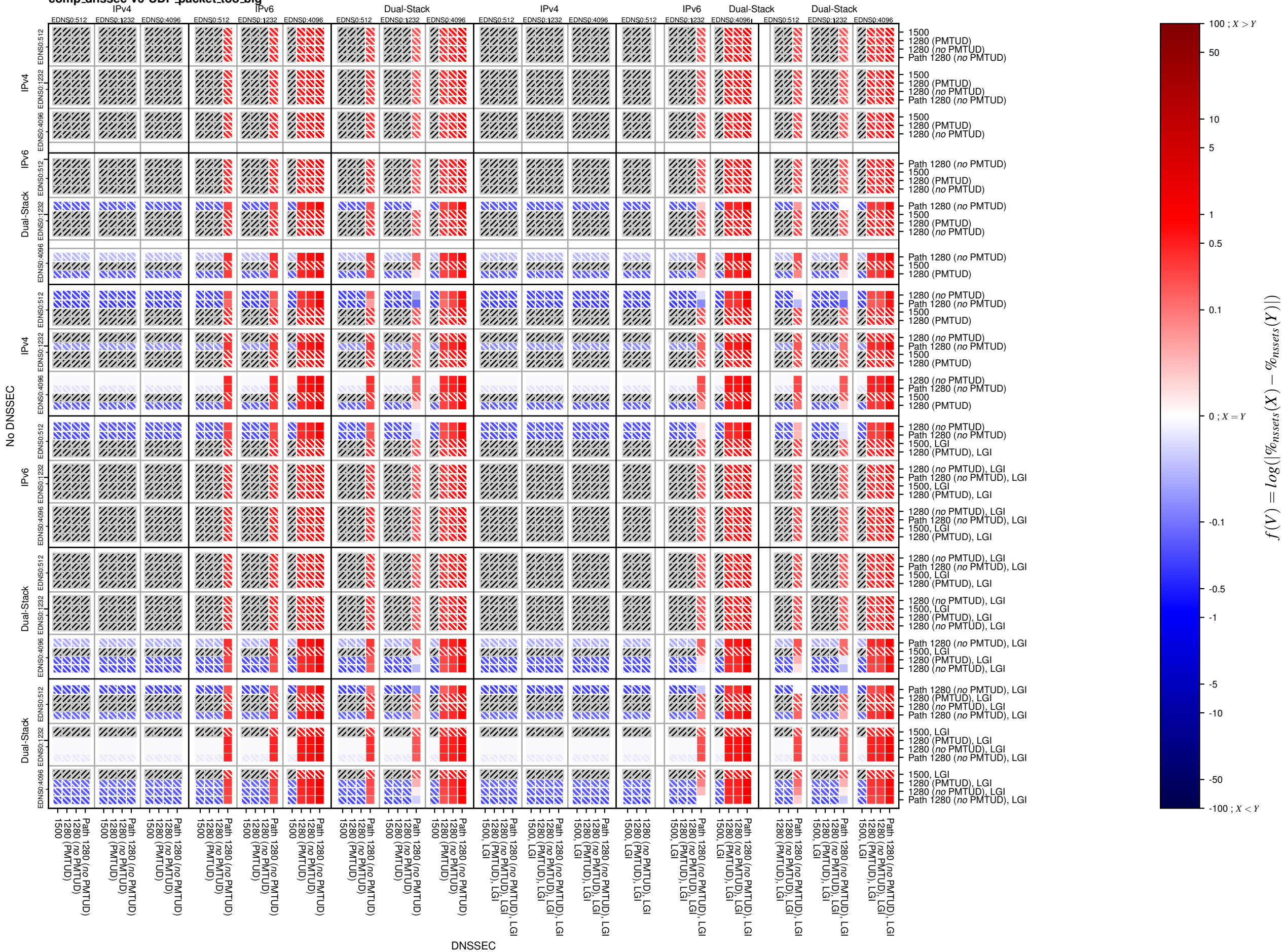
comp_dnsssec-v6-UDP_packet_too_big
