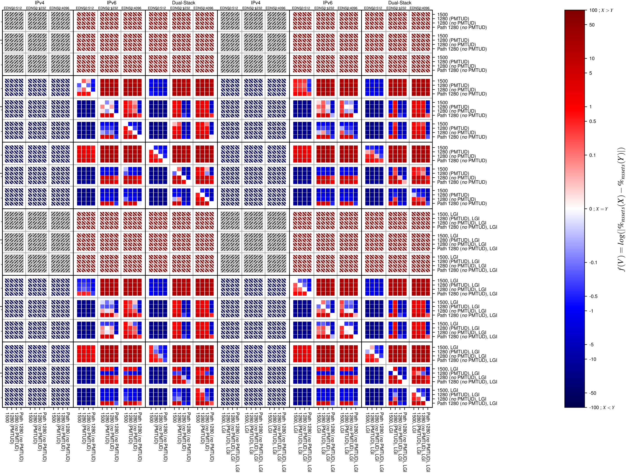
dnssec-v6-UDP_count
