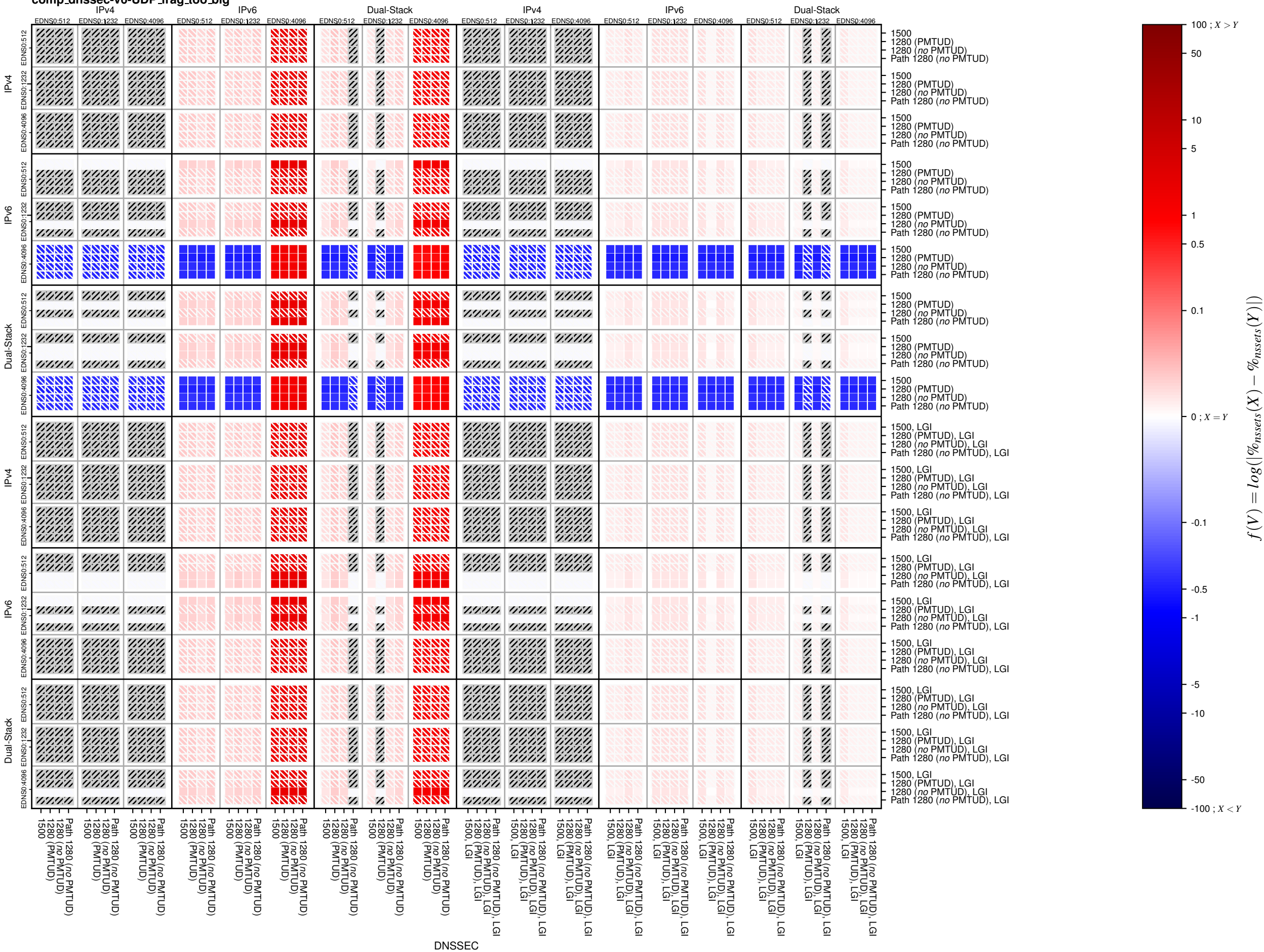
comp_dnssec-v6-UDP_frag_too_big
