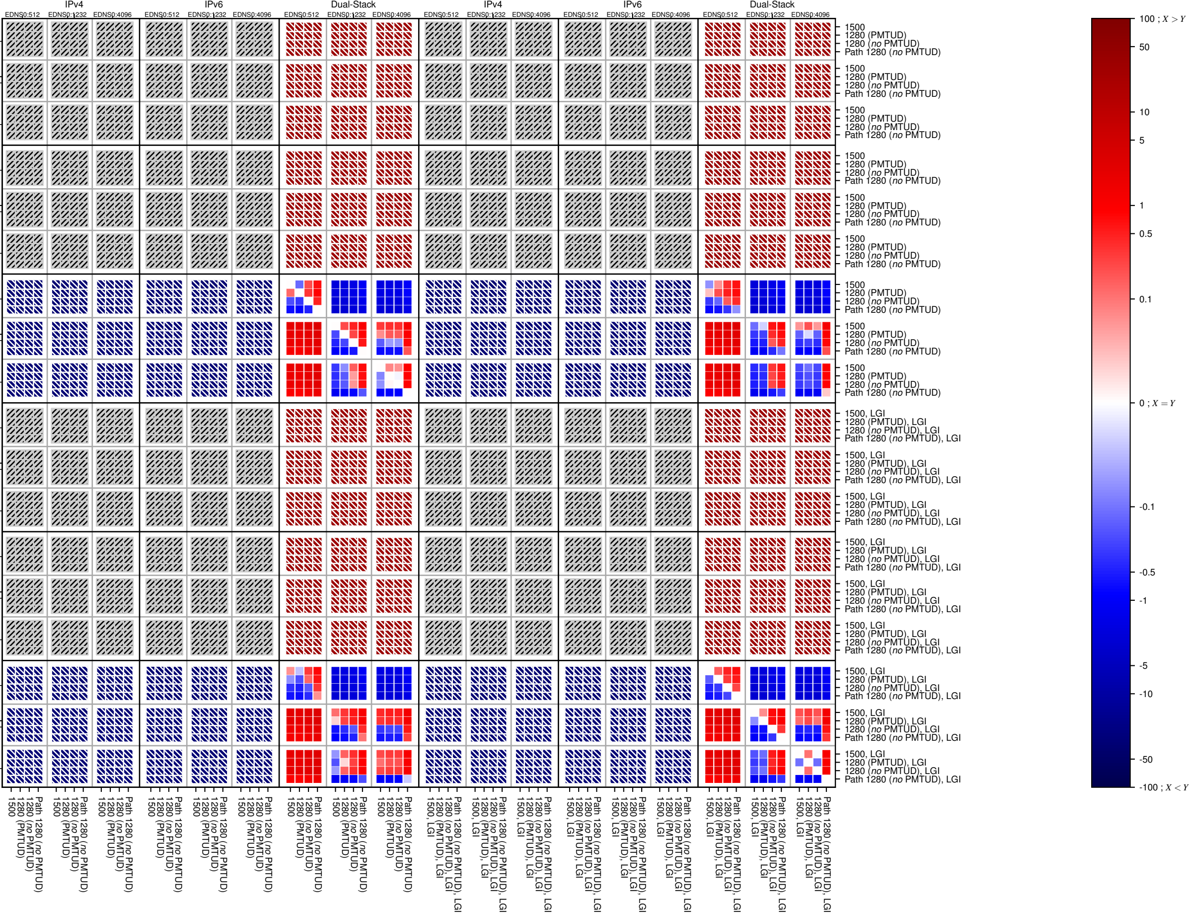
dnssec-v6-UDP_TCP_afi_count
