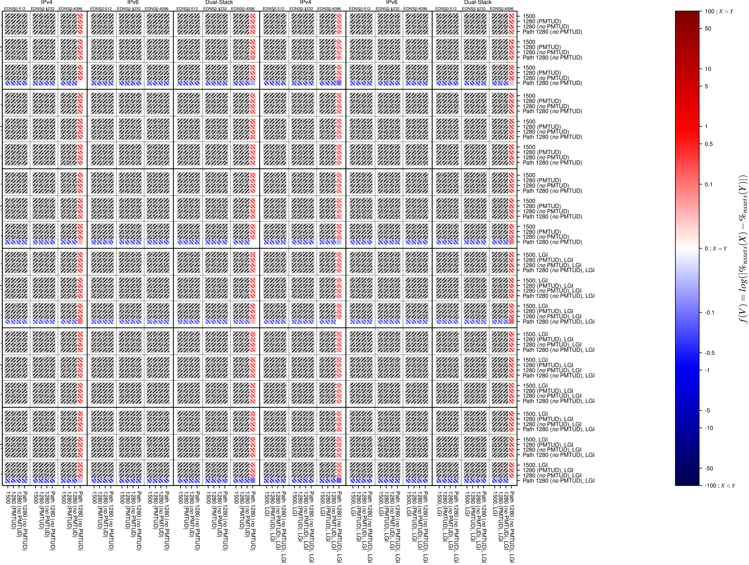
dnssec-v4-TCP_frag_too_big
