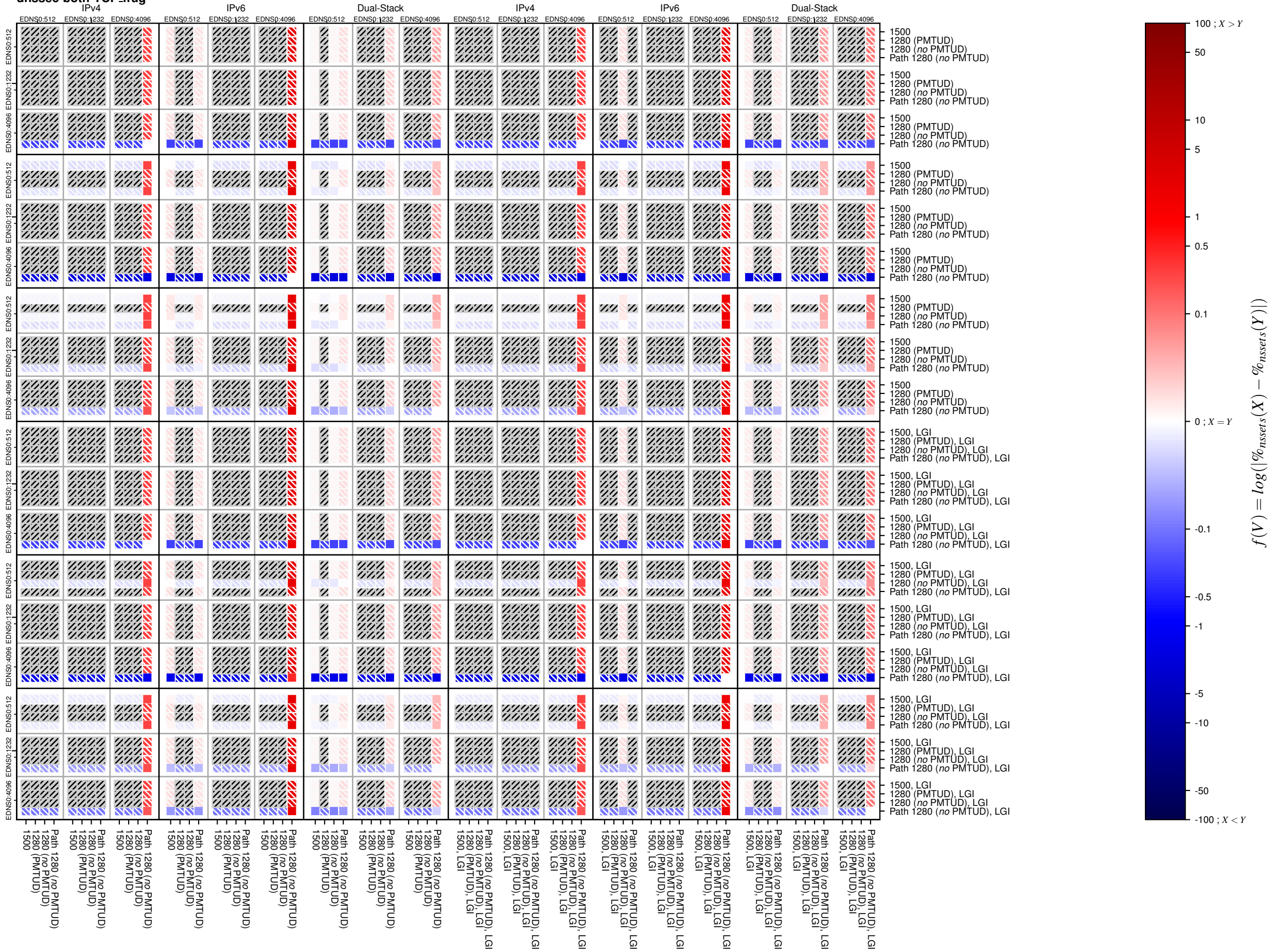
dnssec-both-TCP_frag
