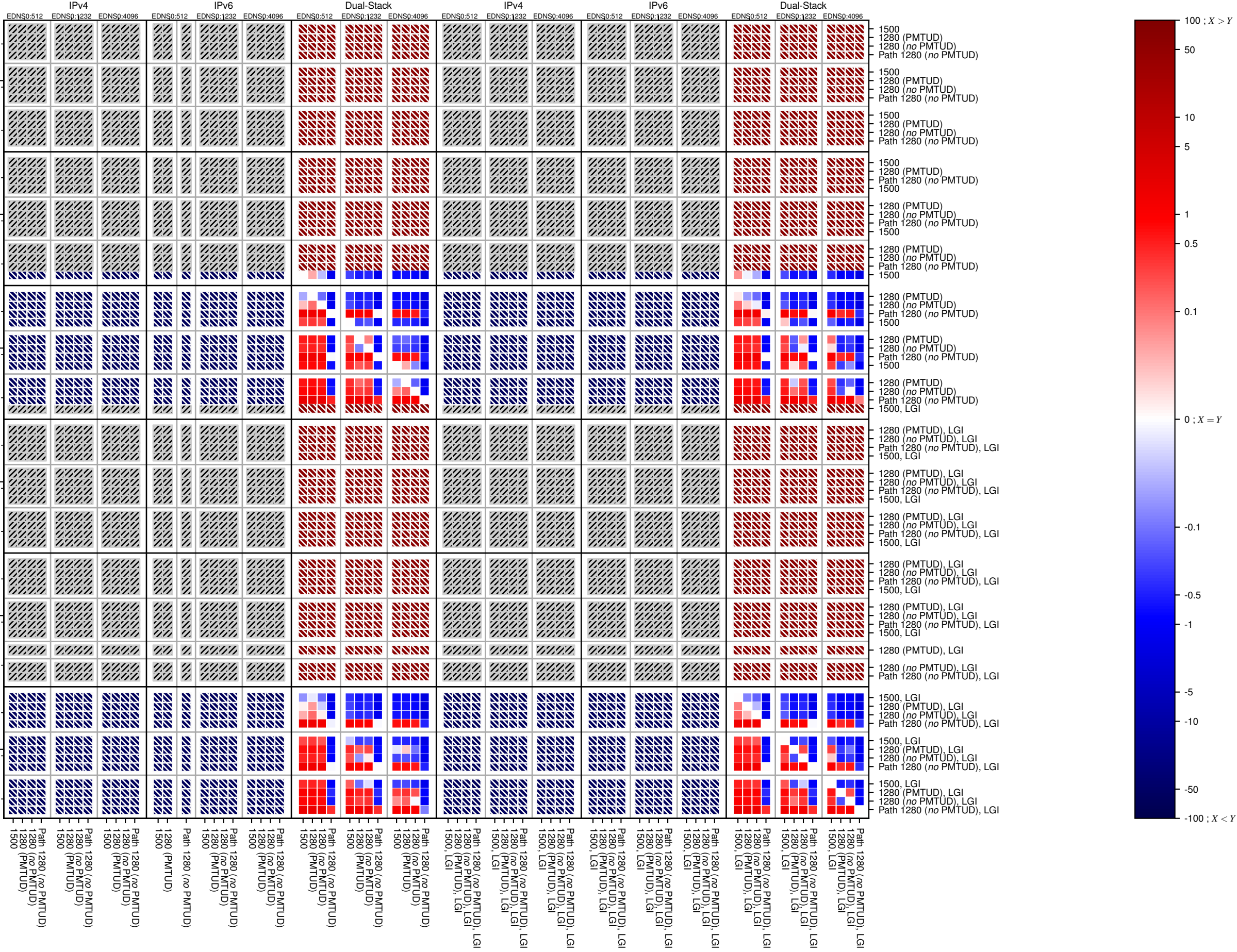
dnssec-v4-UDP_TCP_afi_count
