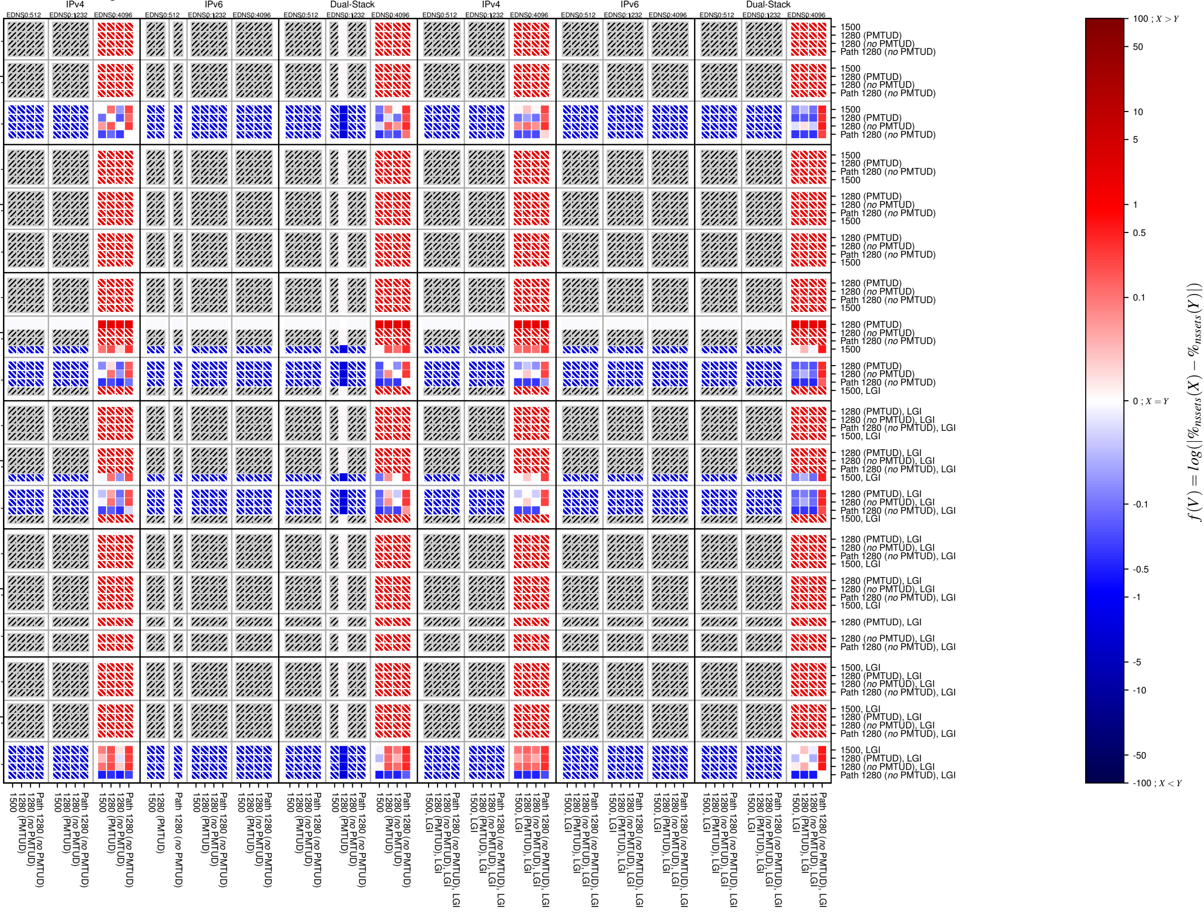
dnssec-v4-UDP_frag
