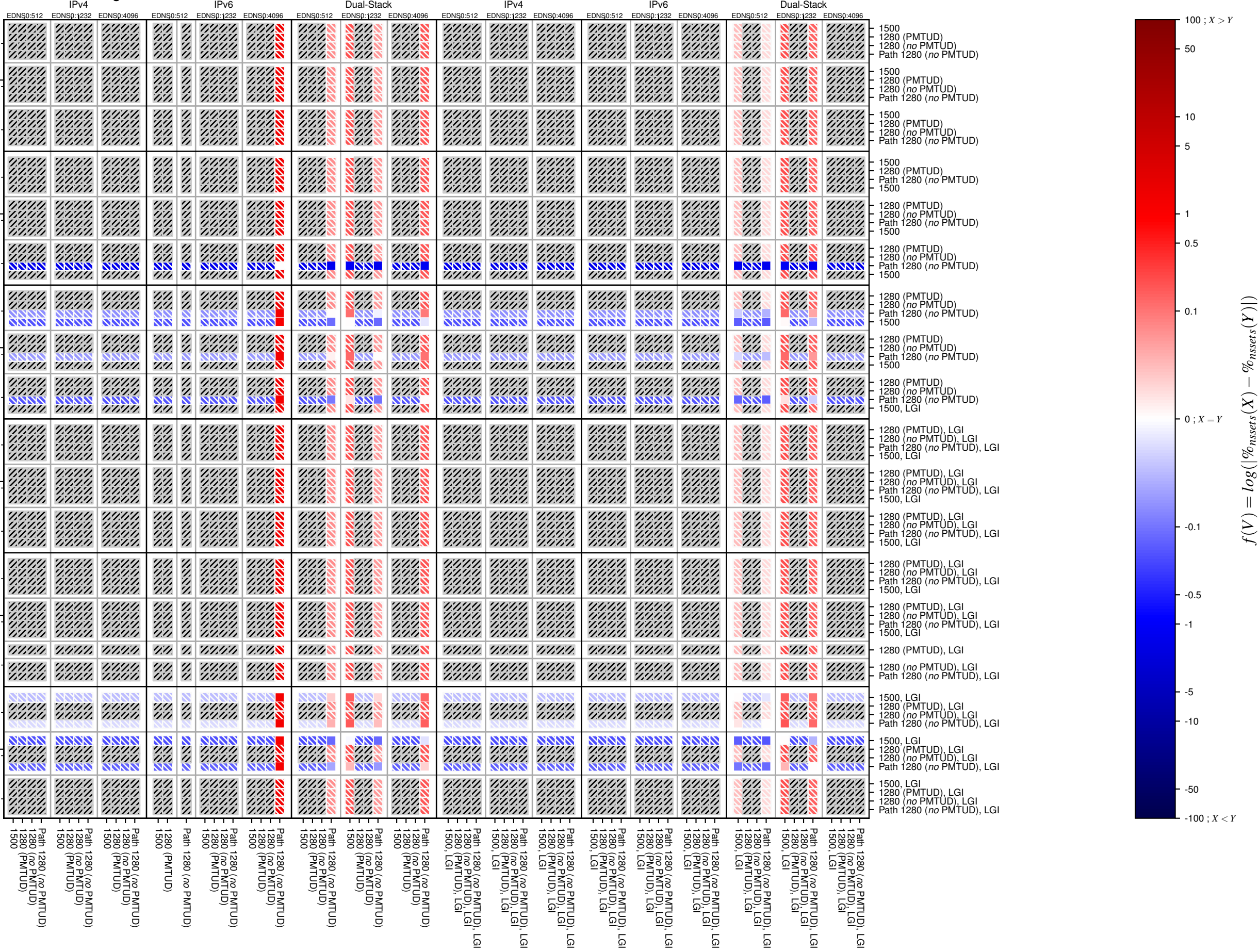
dnssec-v6-TCP_frag
