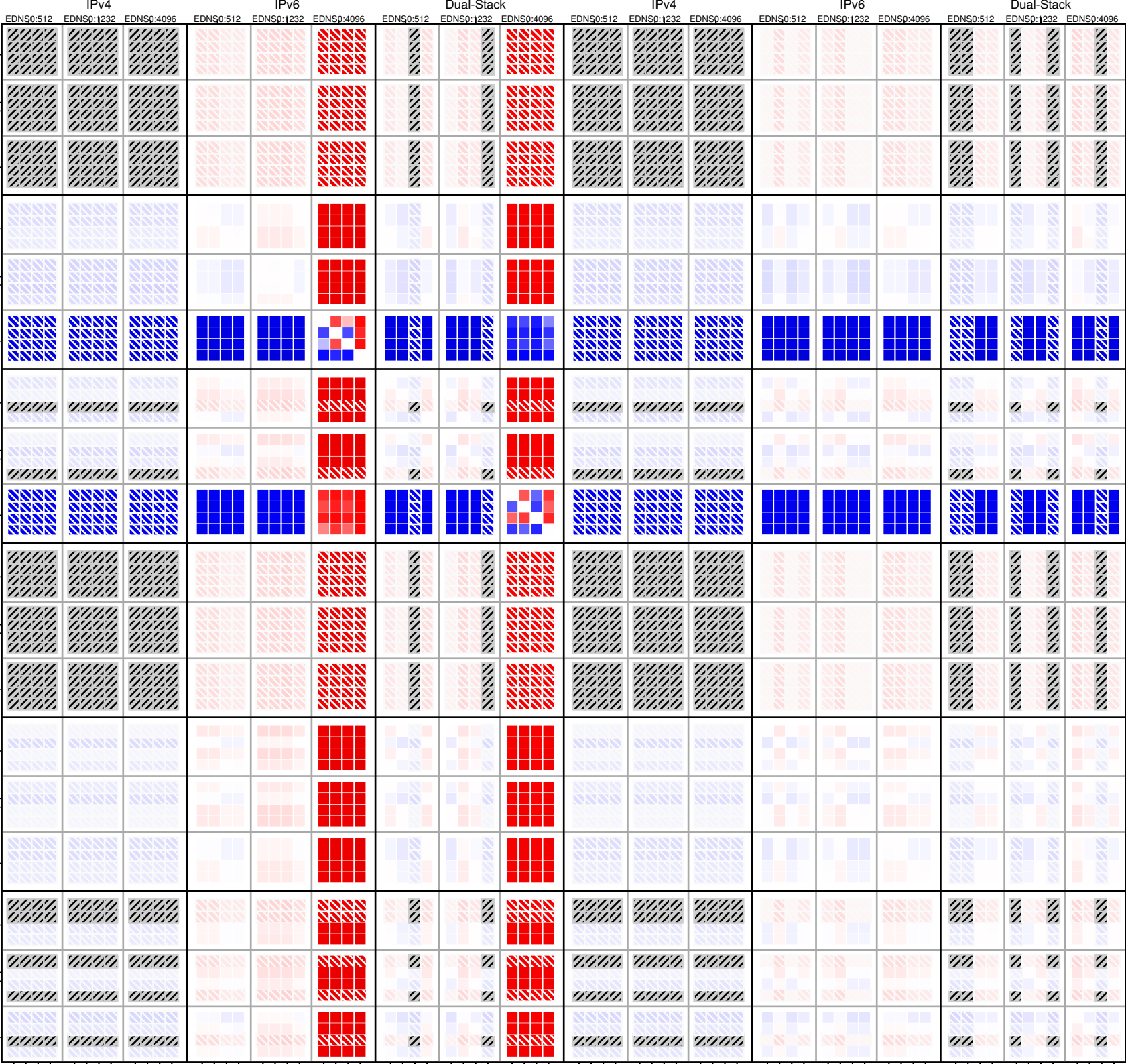
dnssec-v6-UDP_frag.too.big
