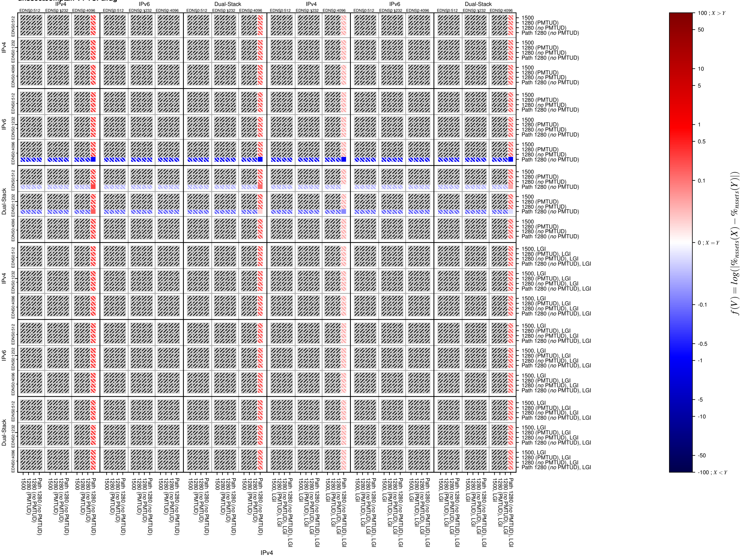
dnssec_comp_afv4-TCP_frag
