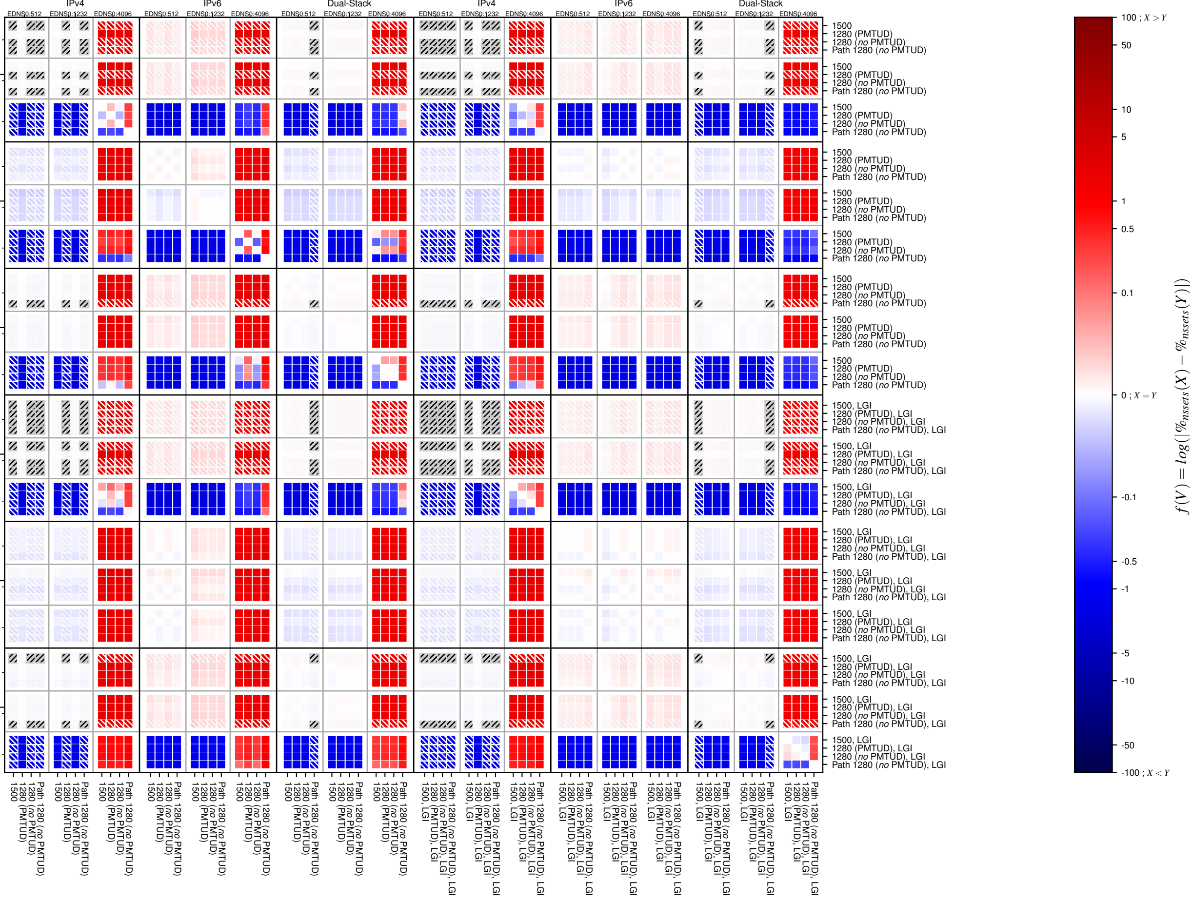
dnssec-both-UDP_frag_too_big
