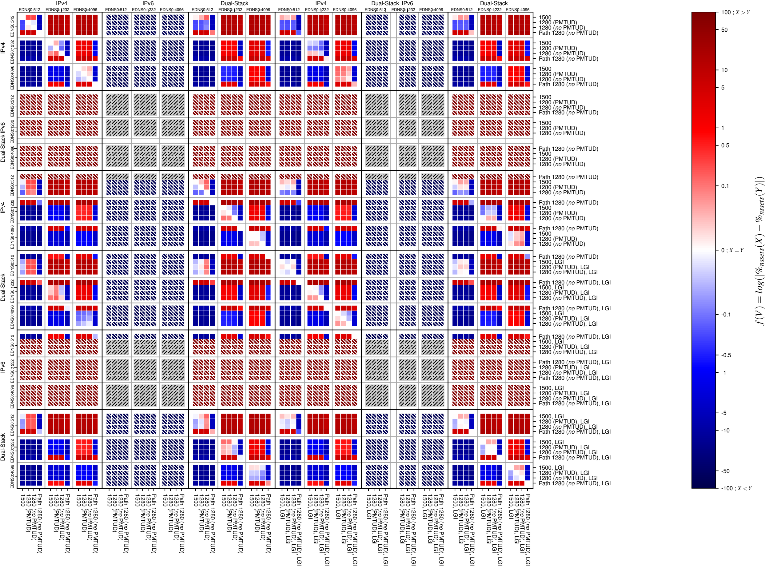
dnssec-v4-UDP_count
