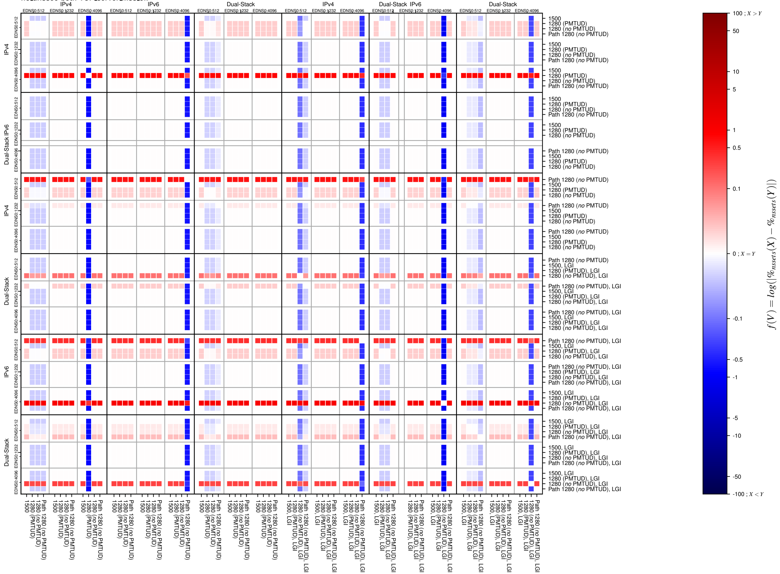
no_dnssec-both-TCP_server_mss_ok
