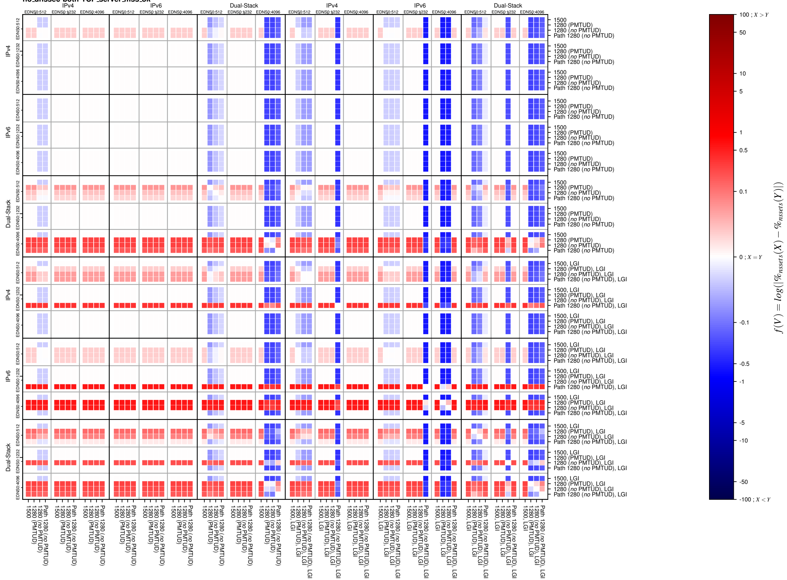
no_dnssec-both-TCP_server_mss_ok
