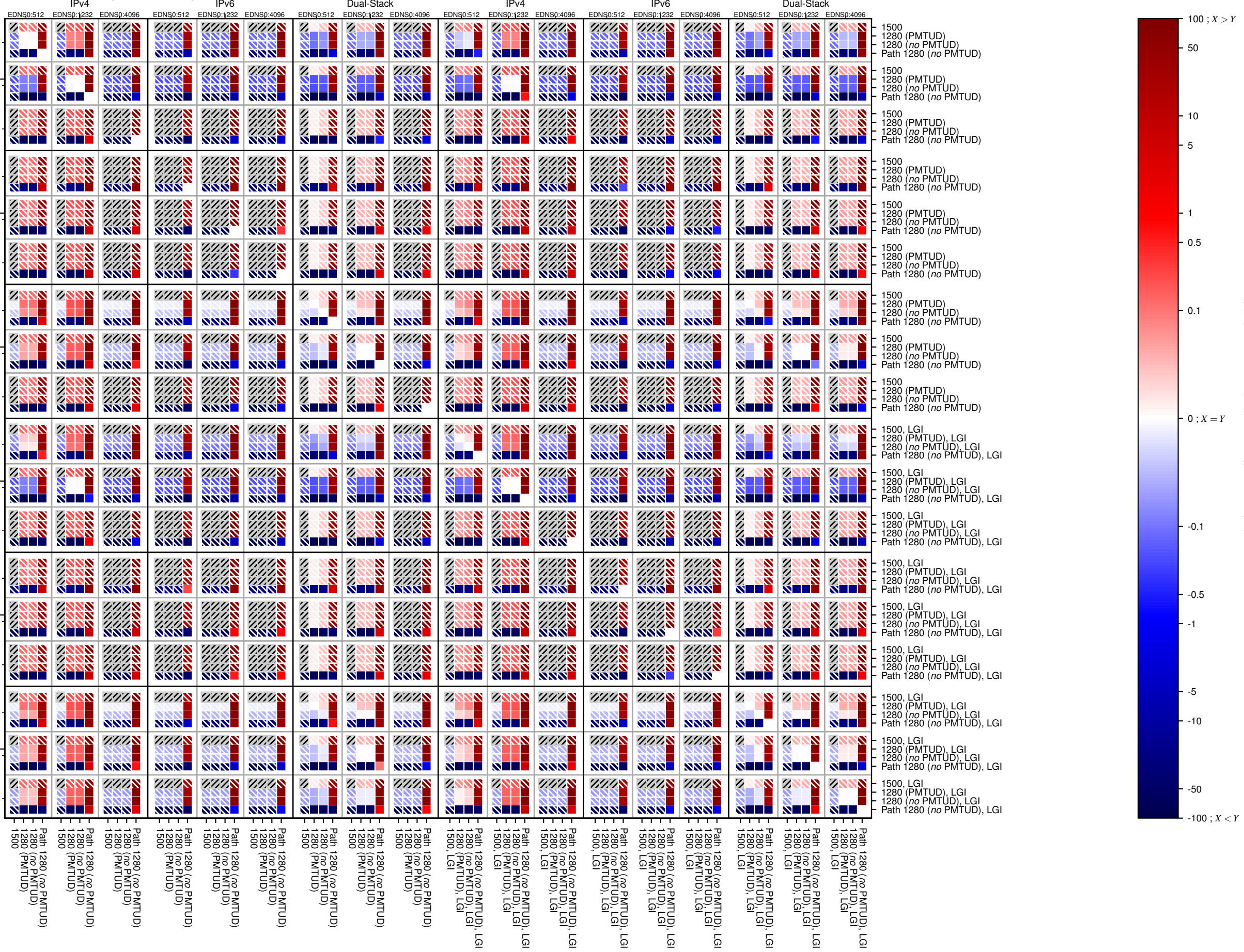
dnssec-both-TCP_packet_too_big
