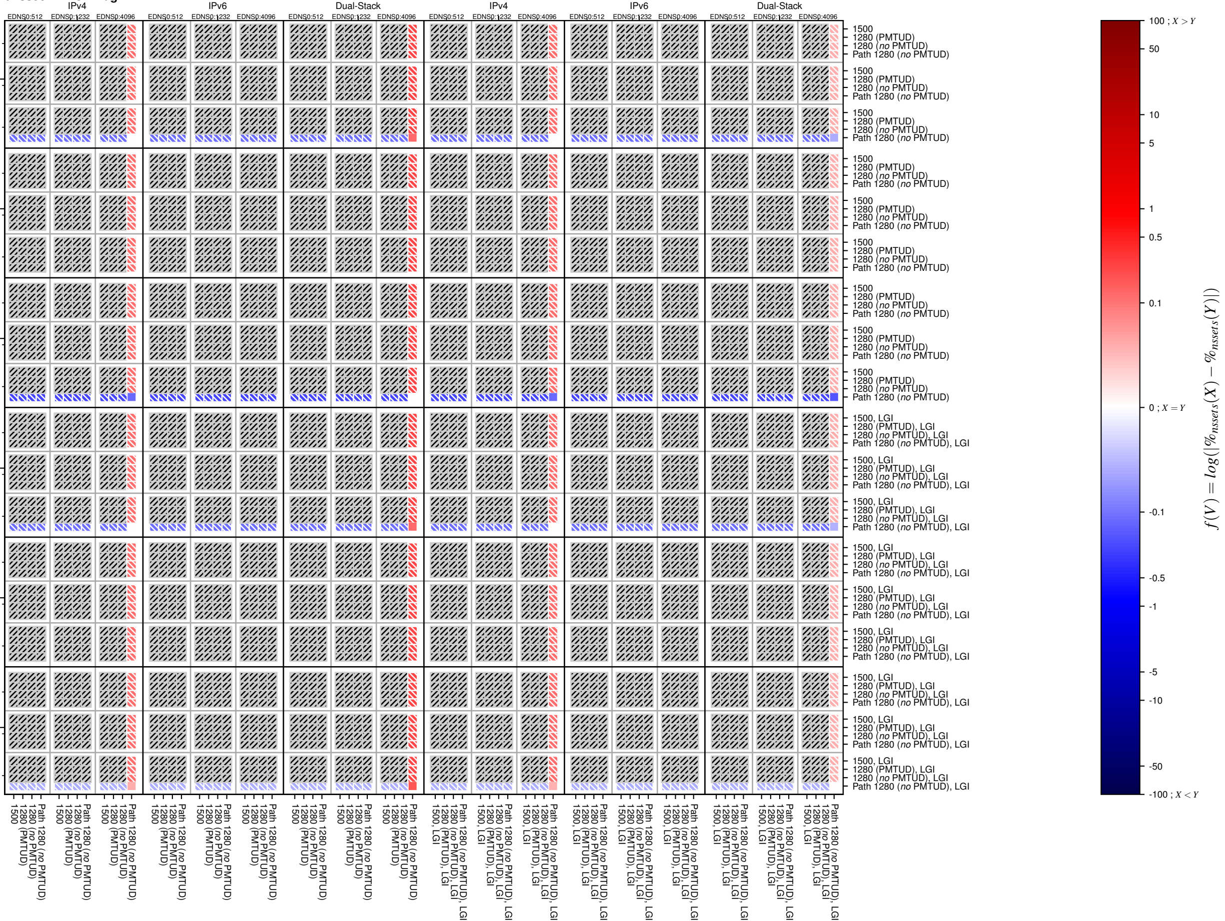
dnssec-v4-TCP_frag
