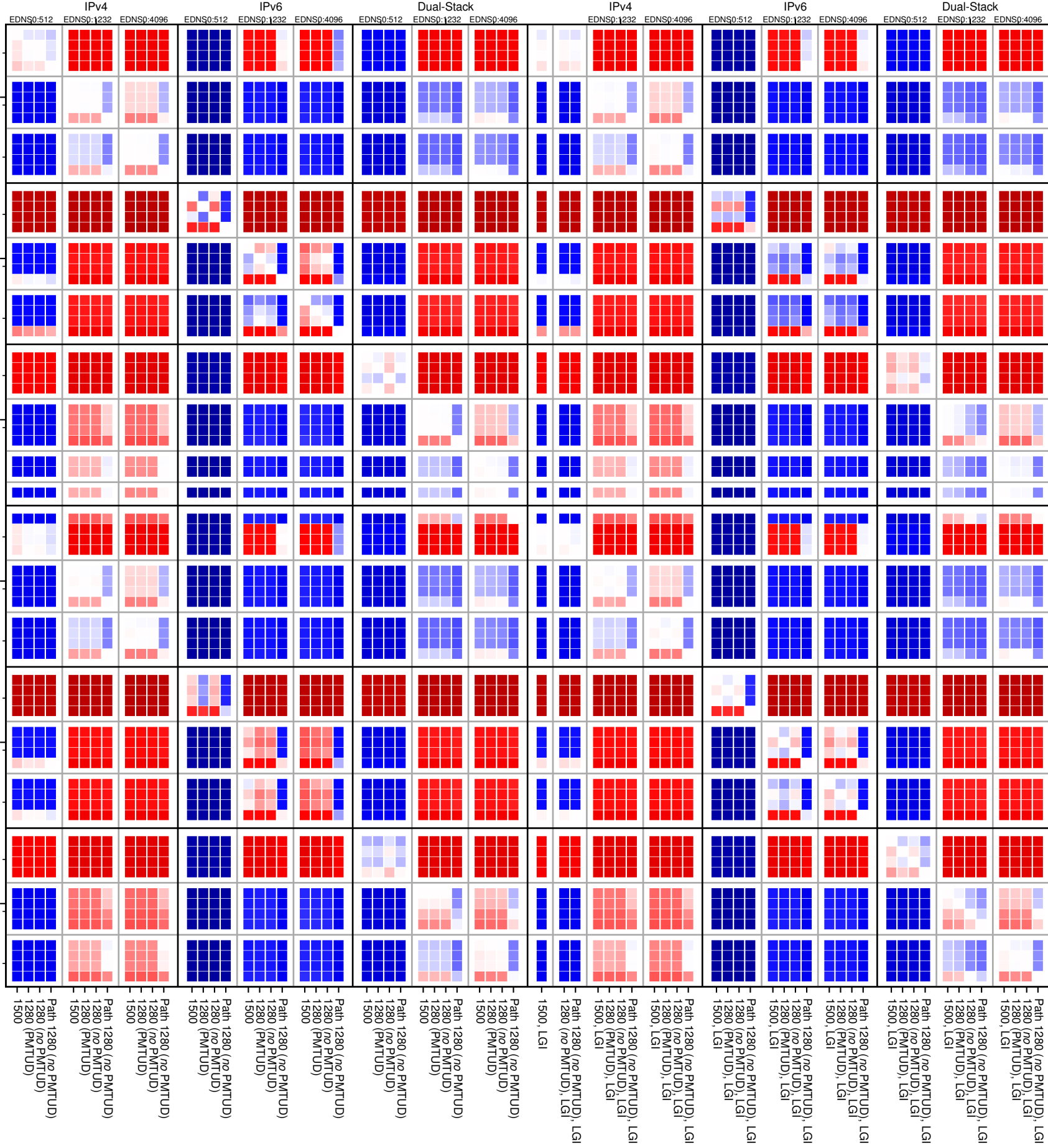
no_dnssec-both-UDP_count
