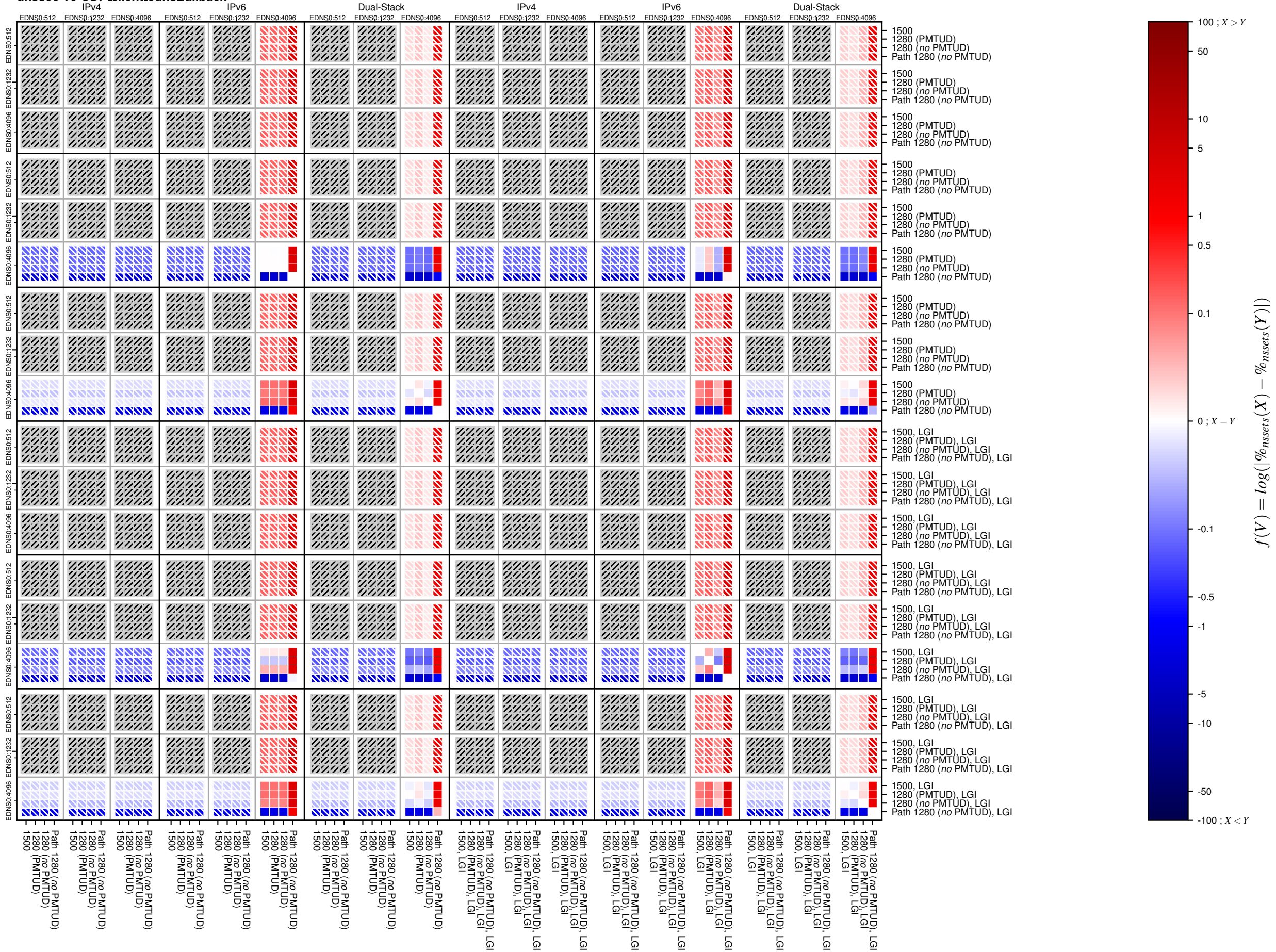
dnssec-v6-UDP_client_edns_fallback
