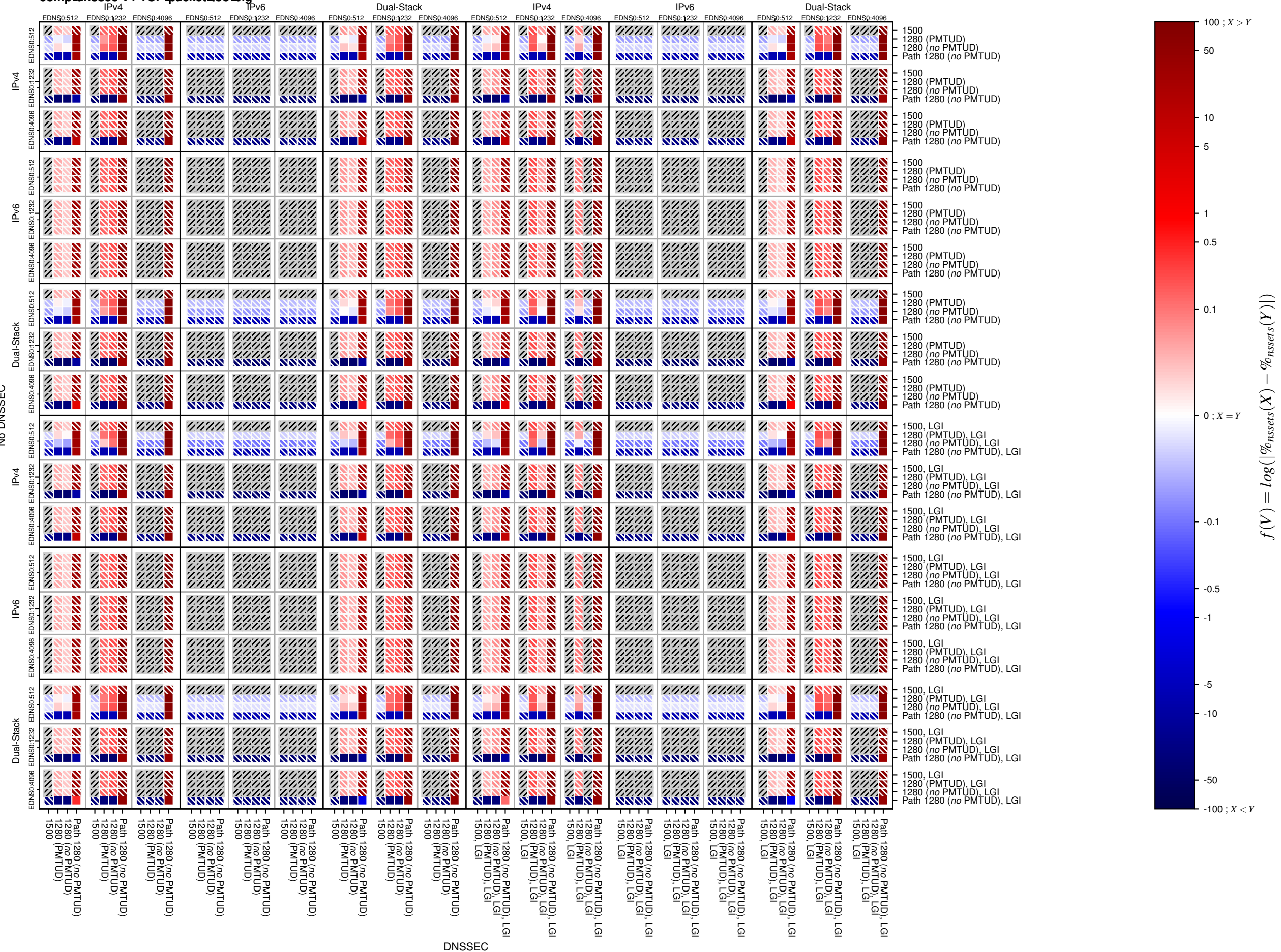
comp_dnssec-v4-TCP_packet_too_big
