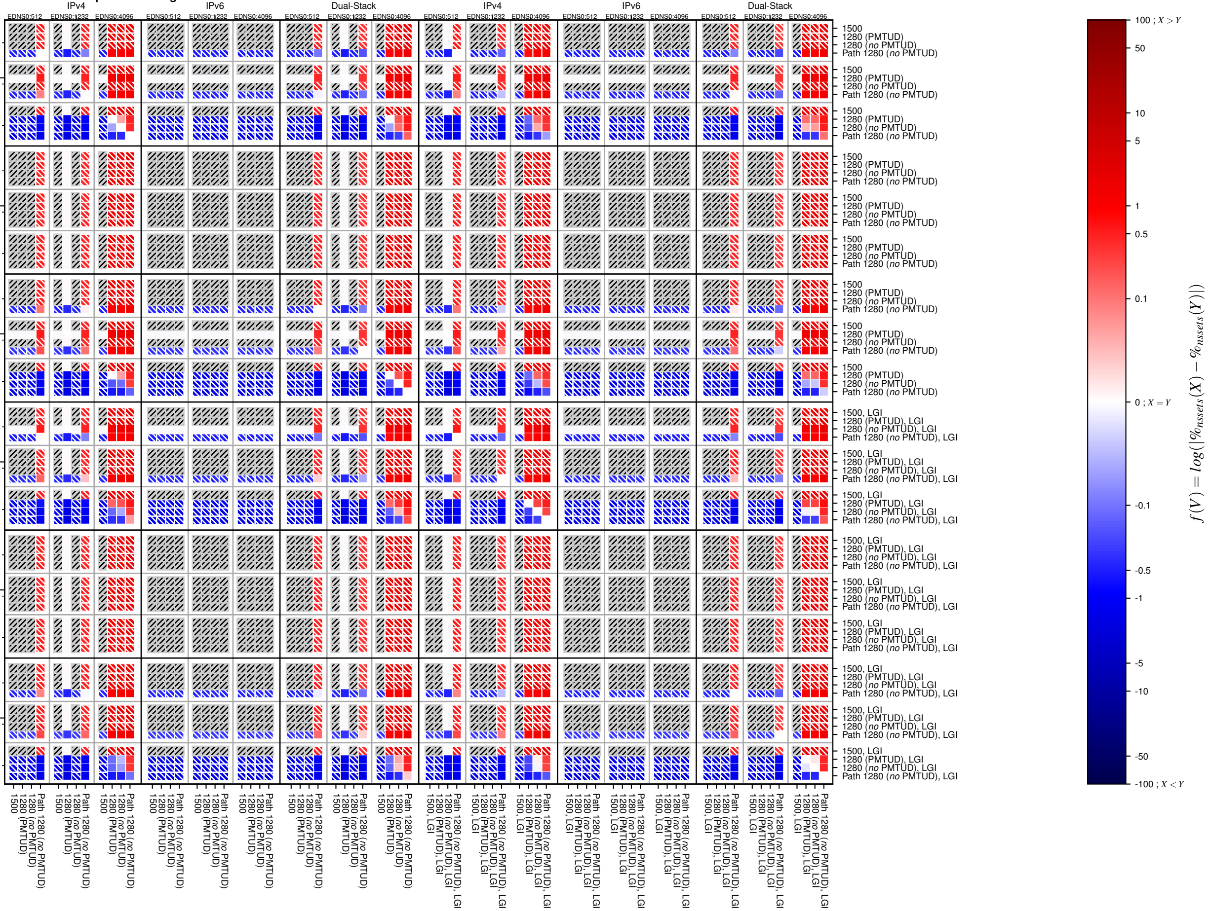
dnssec-v4-UDP_packet_too_big
