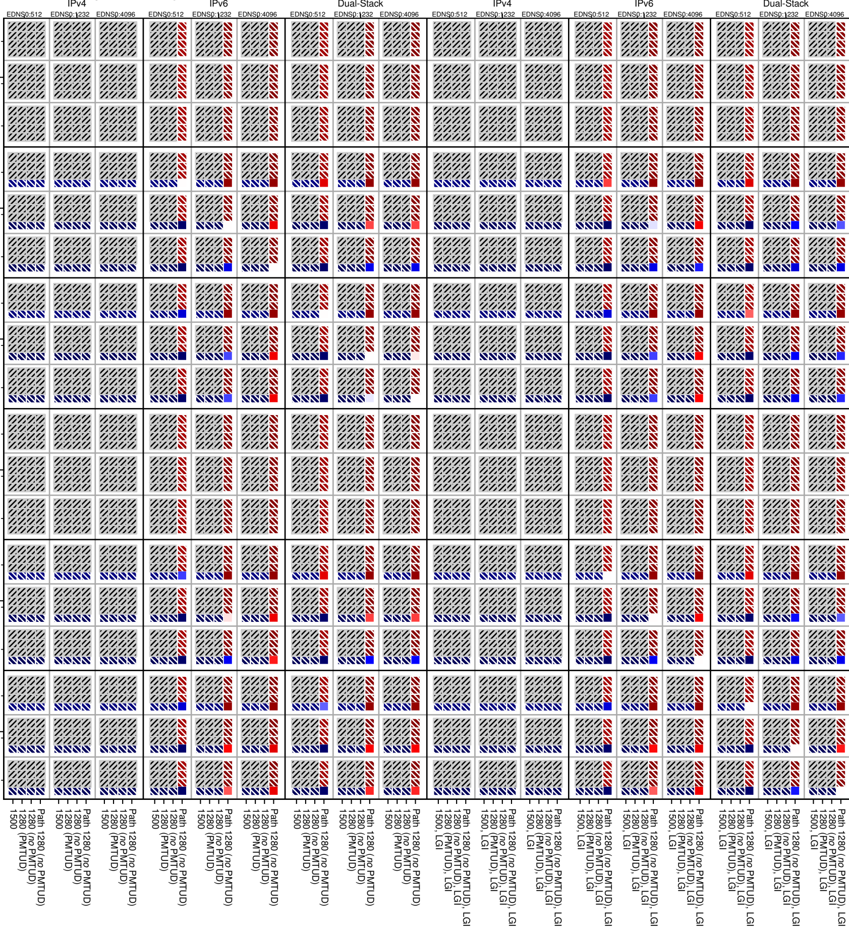
dnssec-v6-TCP_packet_too_big
