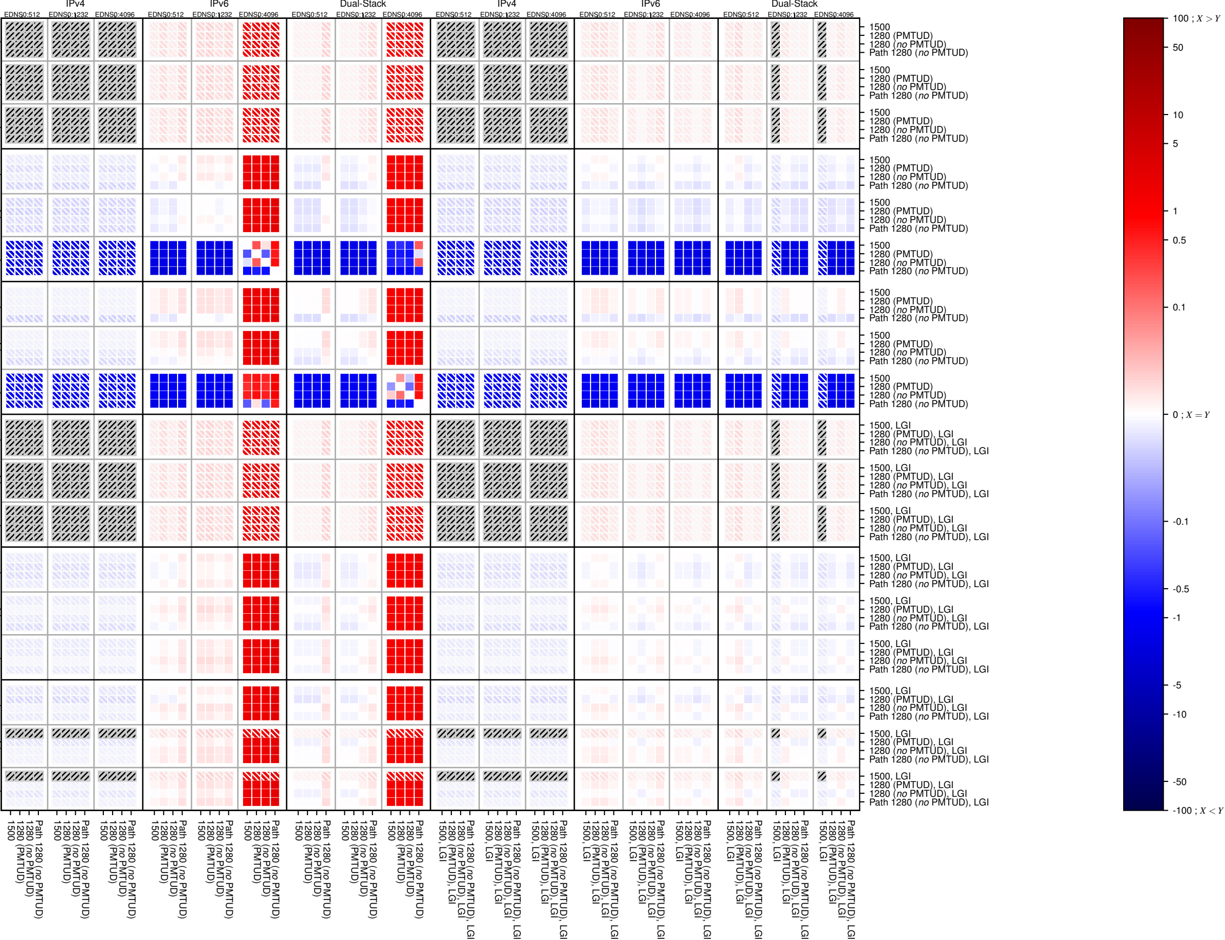
dnssec-v6-UDP_frag.too.big
