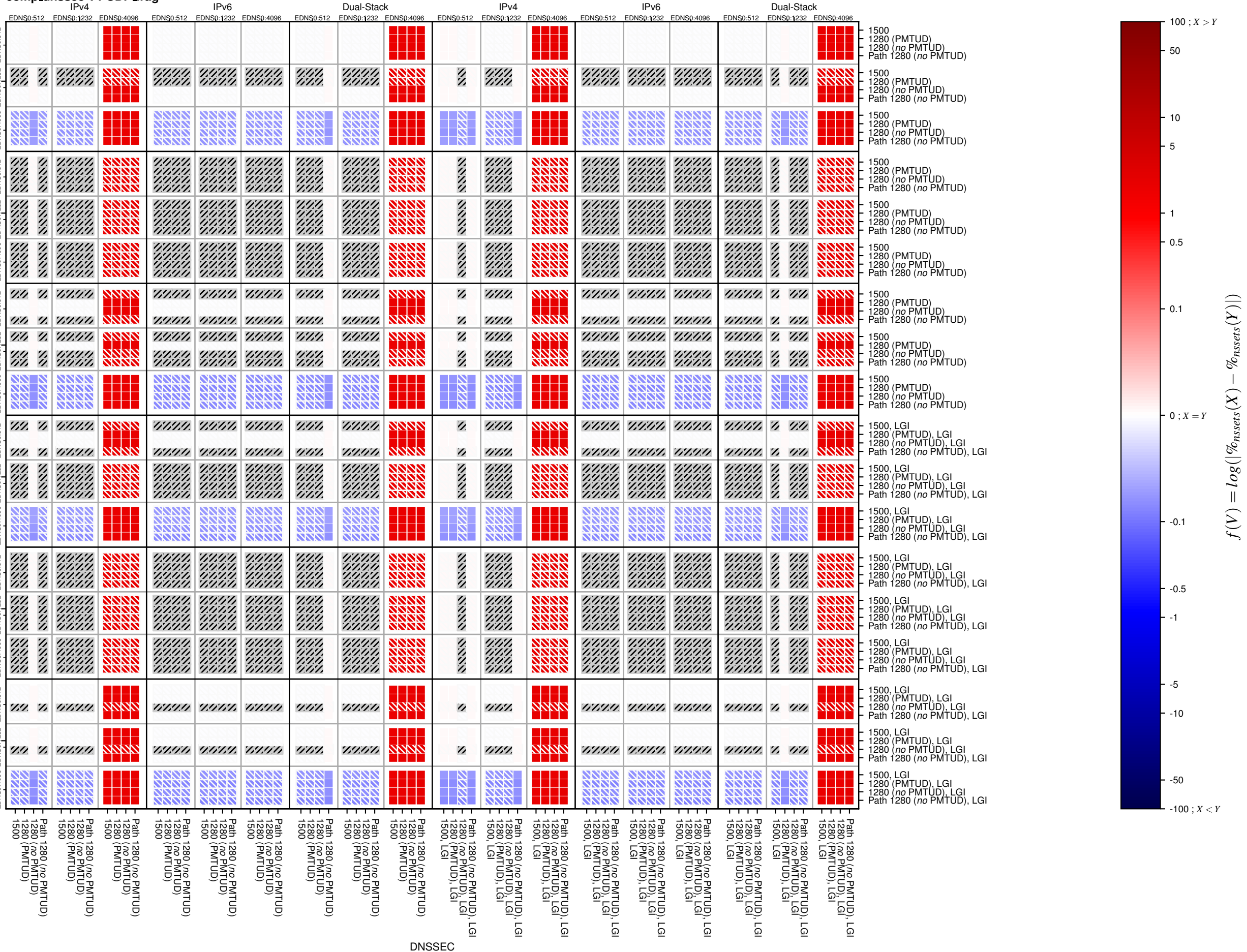
comp_dnssec-v4-UDP_frag
