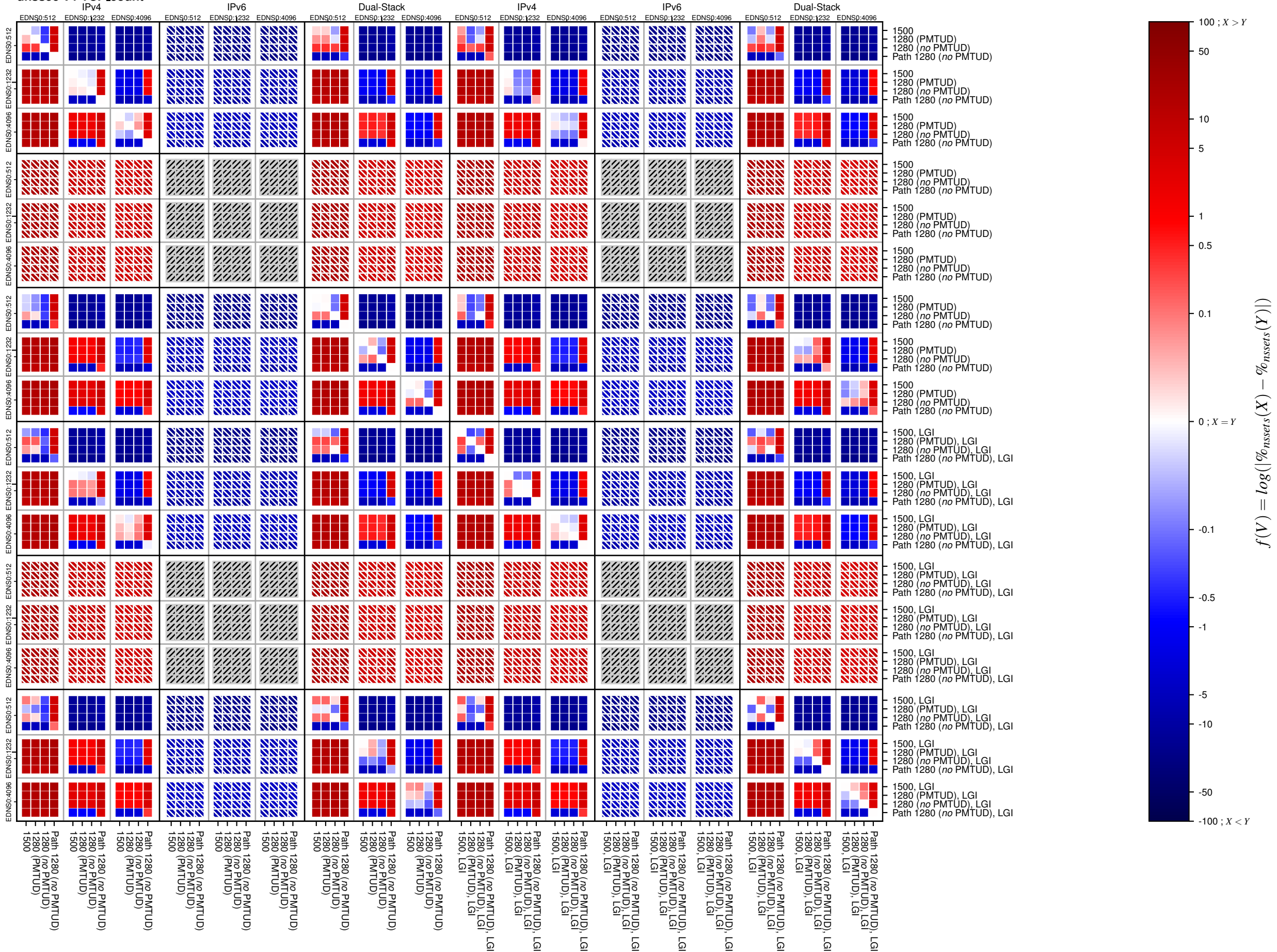
dnssec-v4-TCP_count
