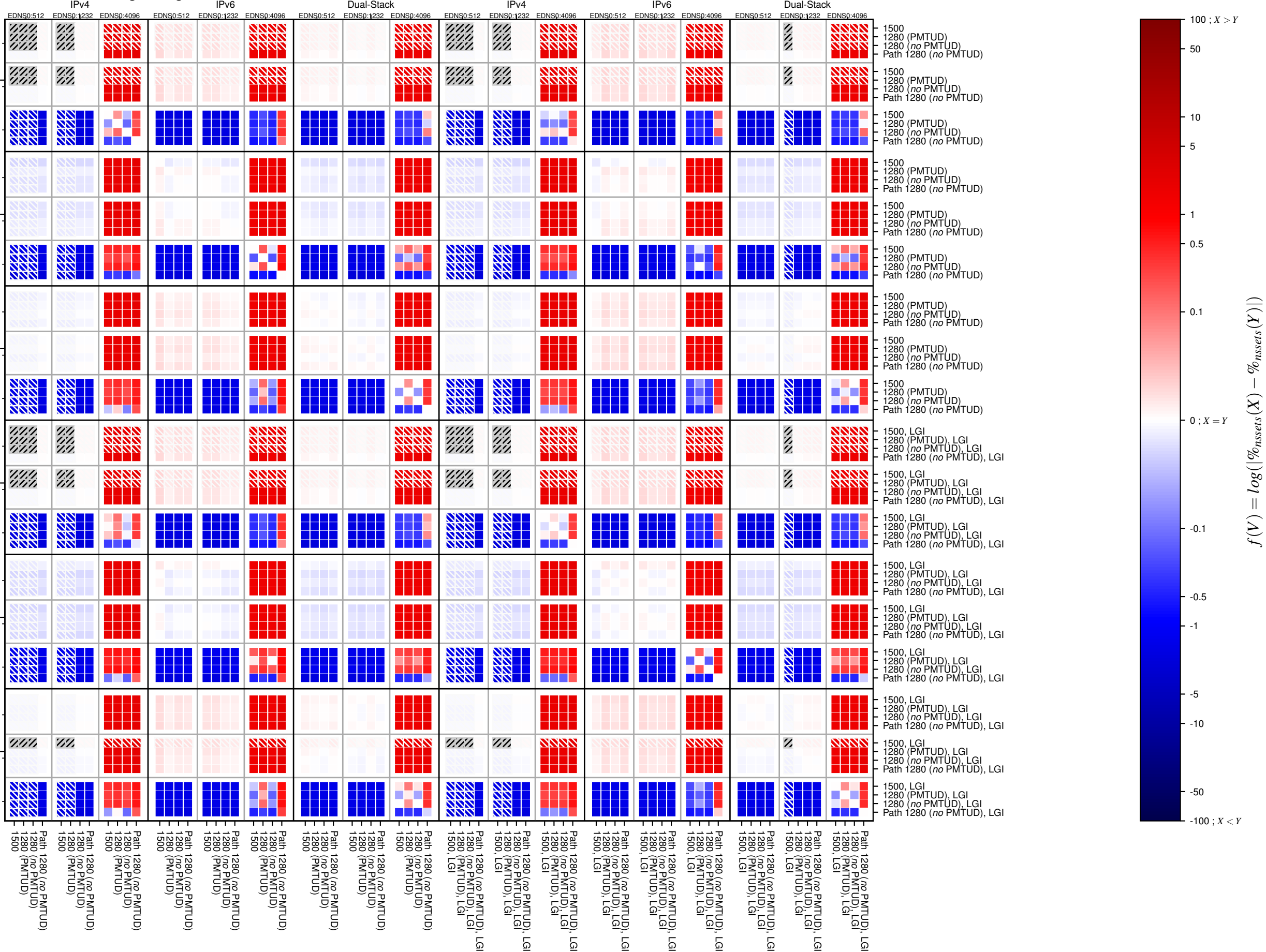
dnssec-both-UDP_frag_too_big
