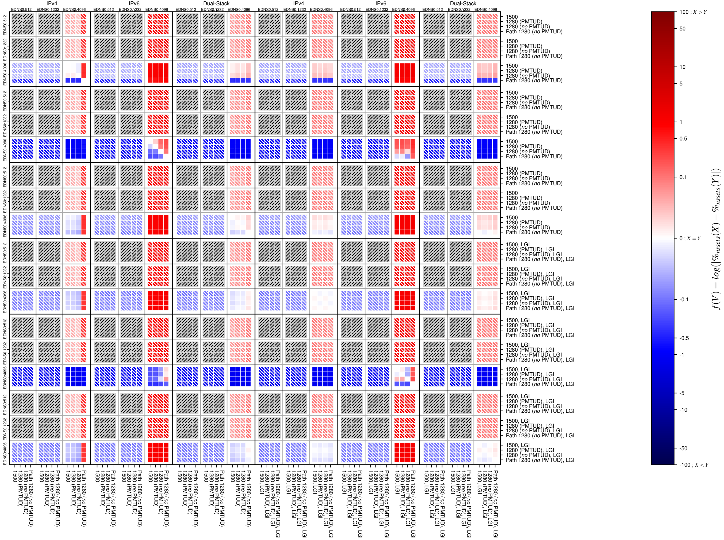
no_dnssec-both-UDP_client_edns_fallback
