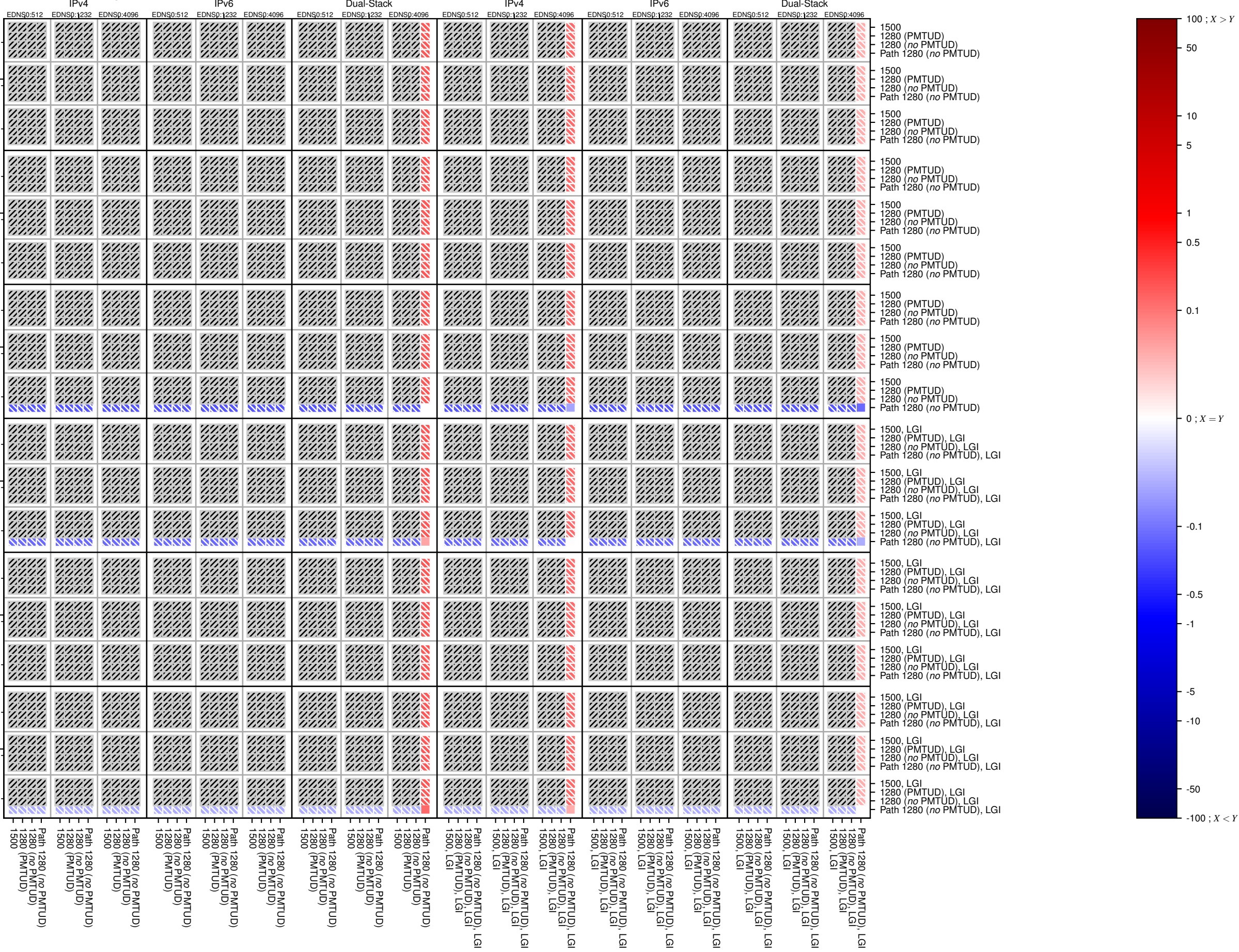
dnssec-v4-TCP_frag
