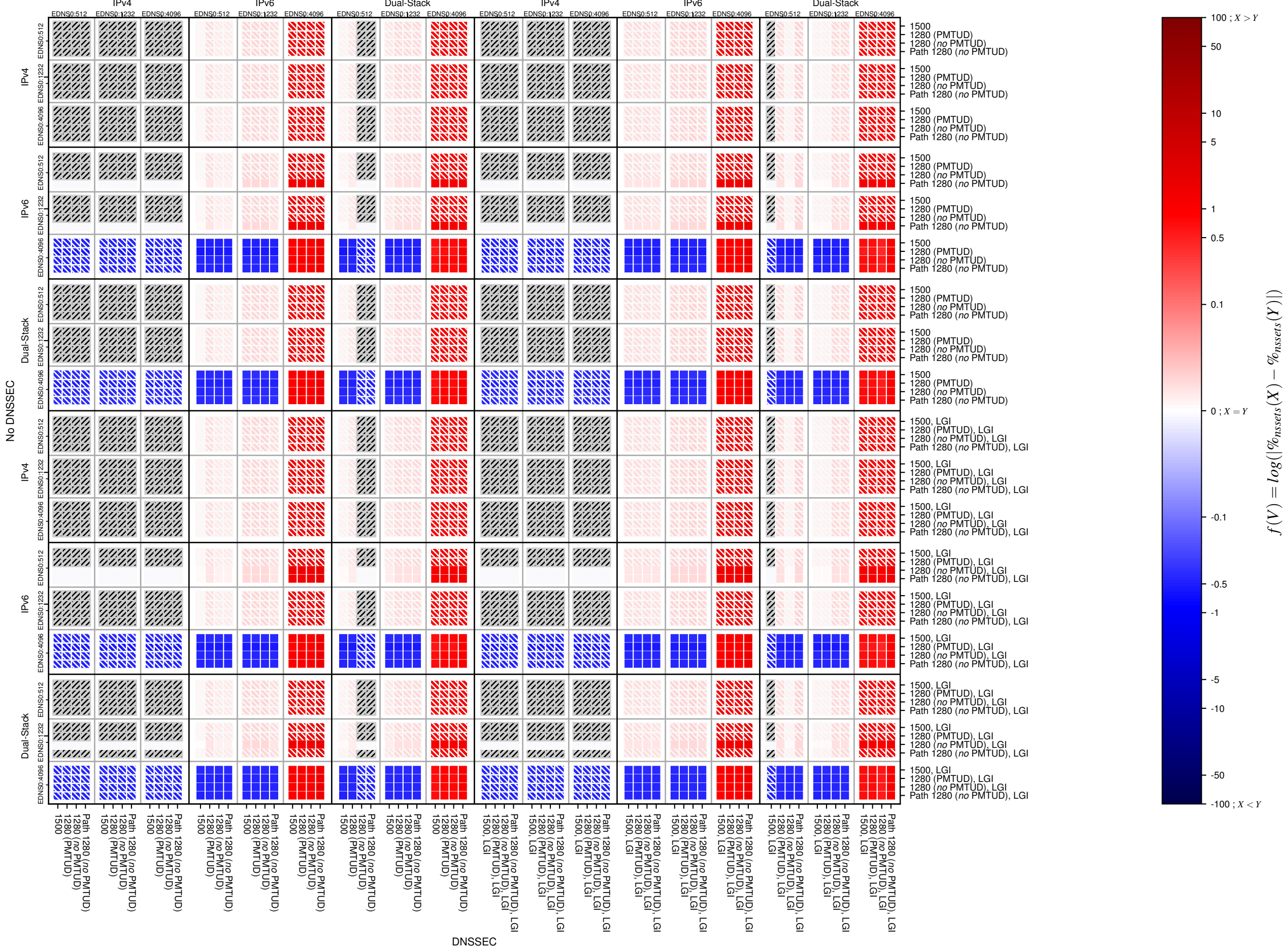
comp_dnssec-v6-UDP_frag_too_big
