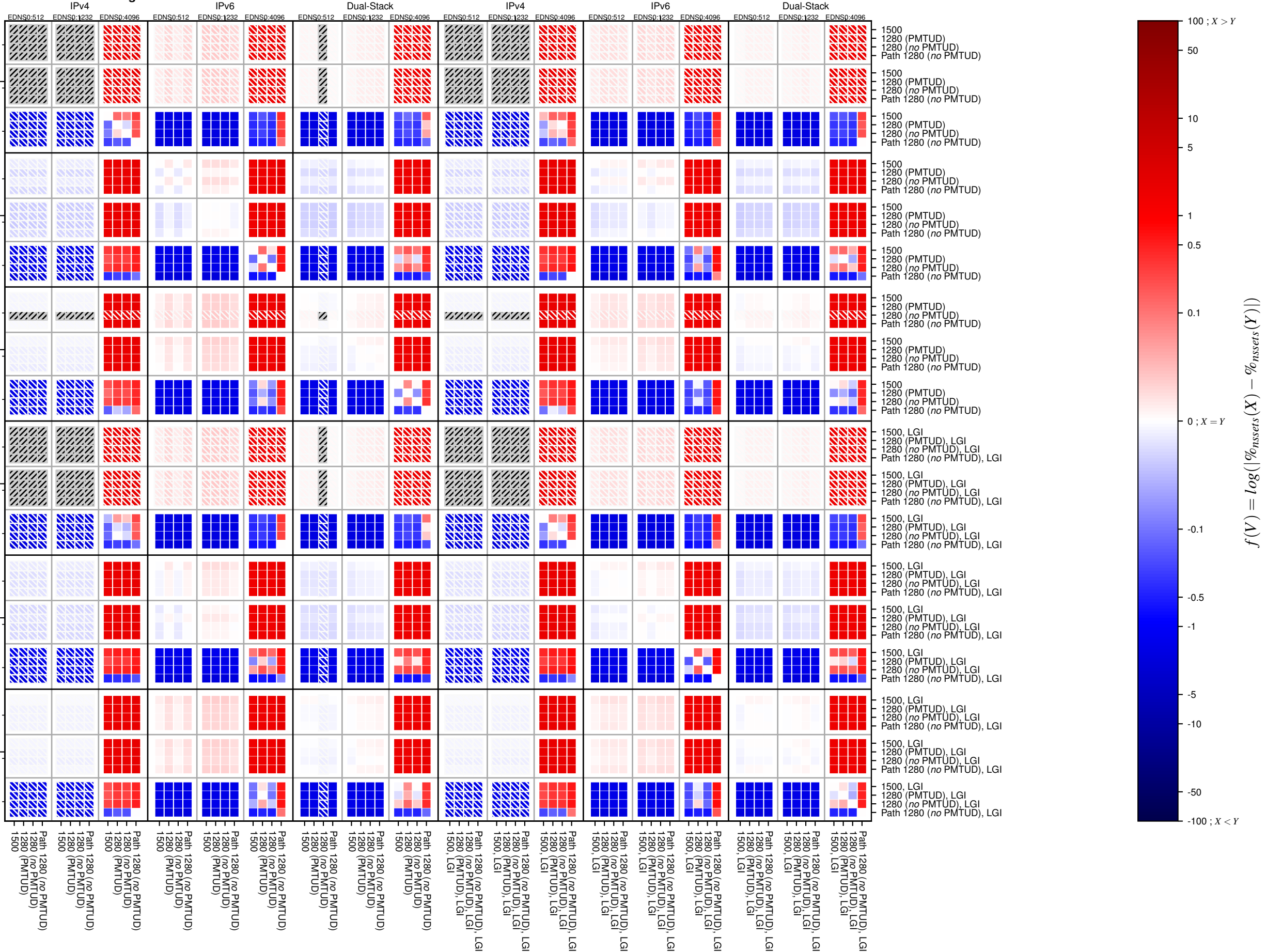
dnssec-both-UDP_frag
