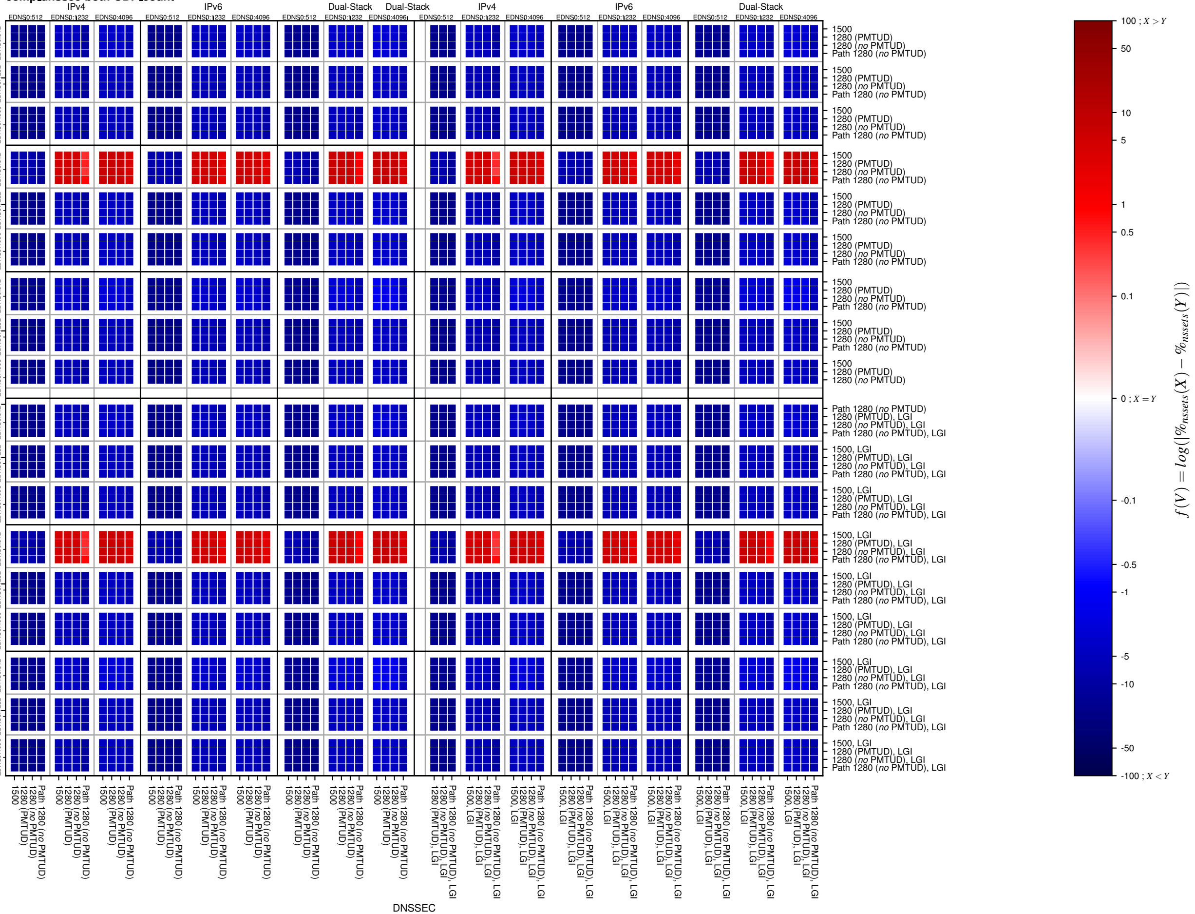
comp_dnssec-both-UDP_count
