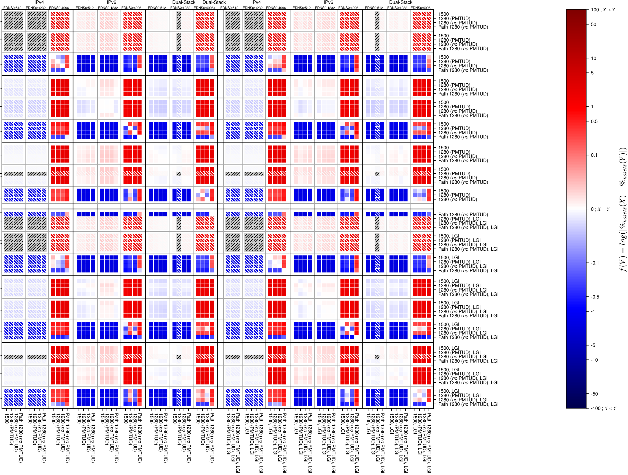
dnssec-both-UDP_frag_too_big
