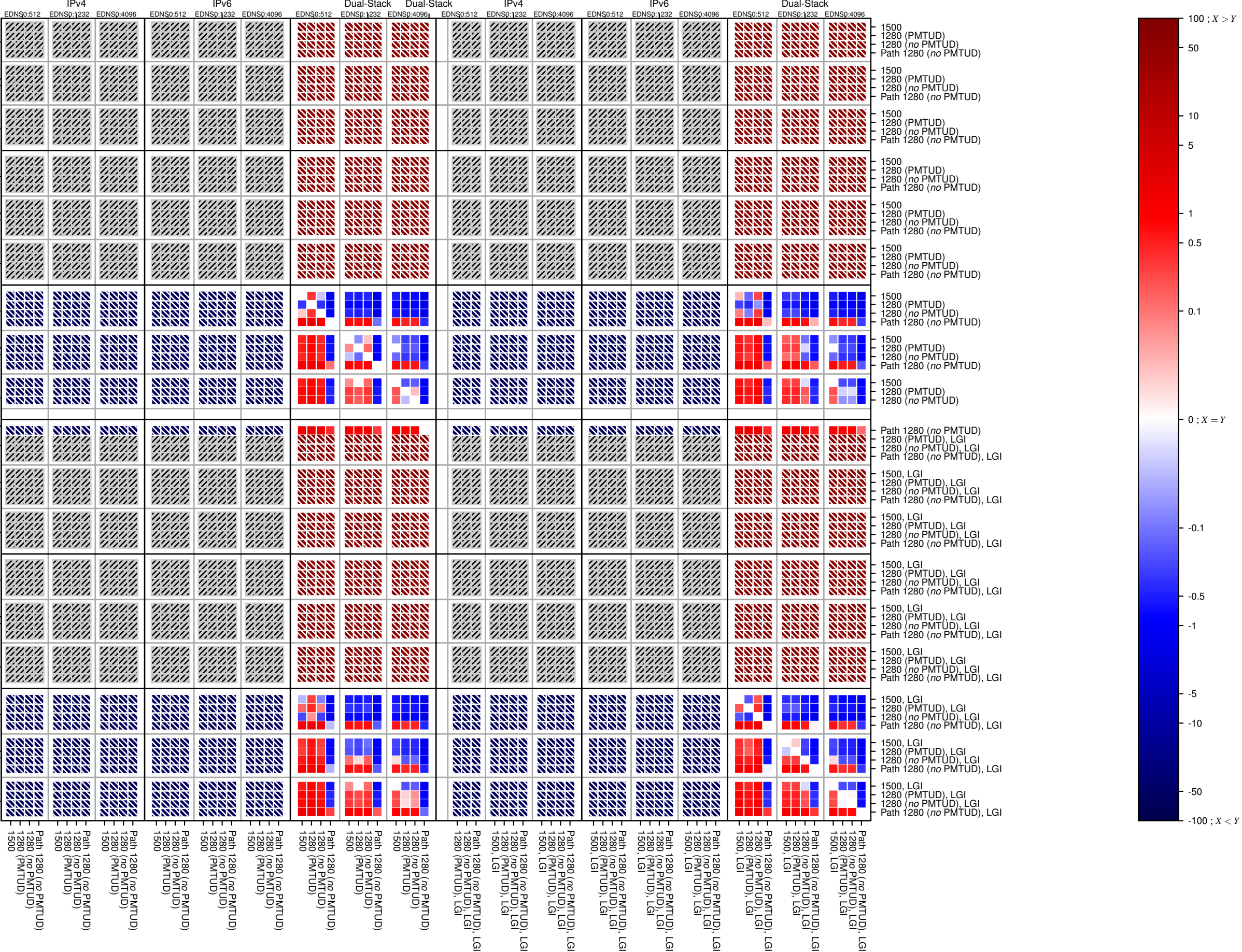
dnssec-v4-UDP_TCP_afi_count
