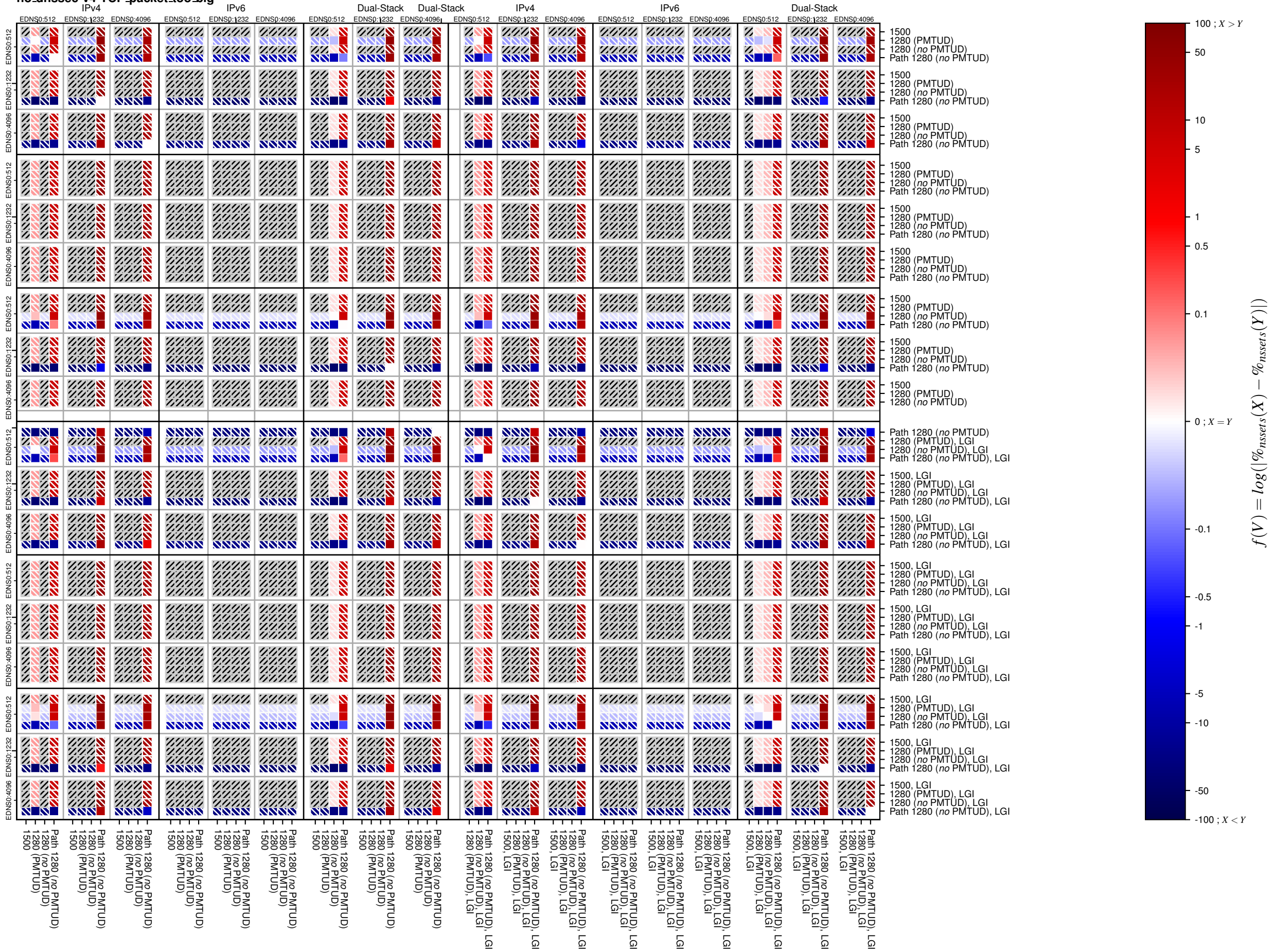
no_dnssec-v4-TCP_packet_too_big
