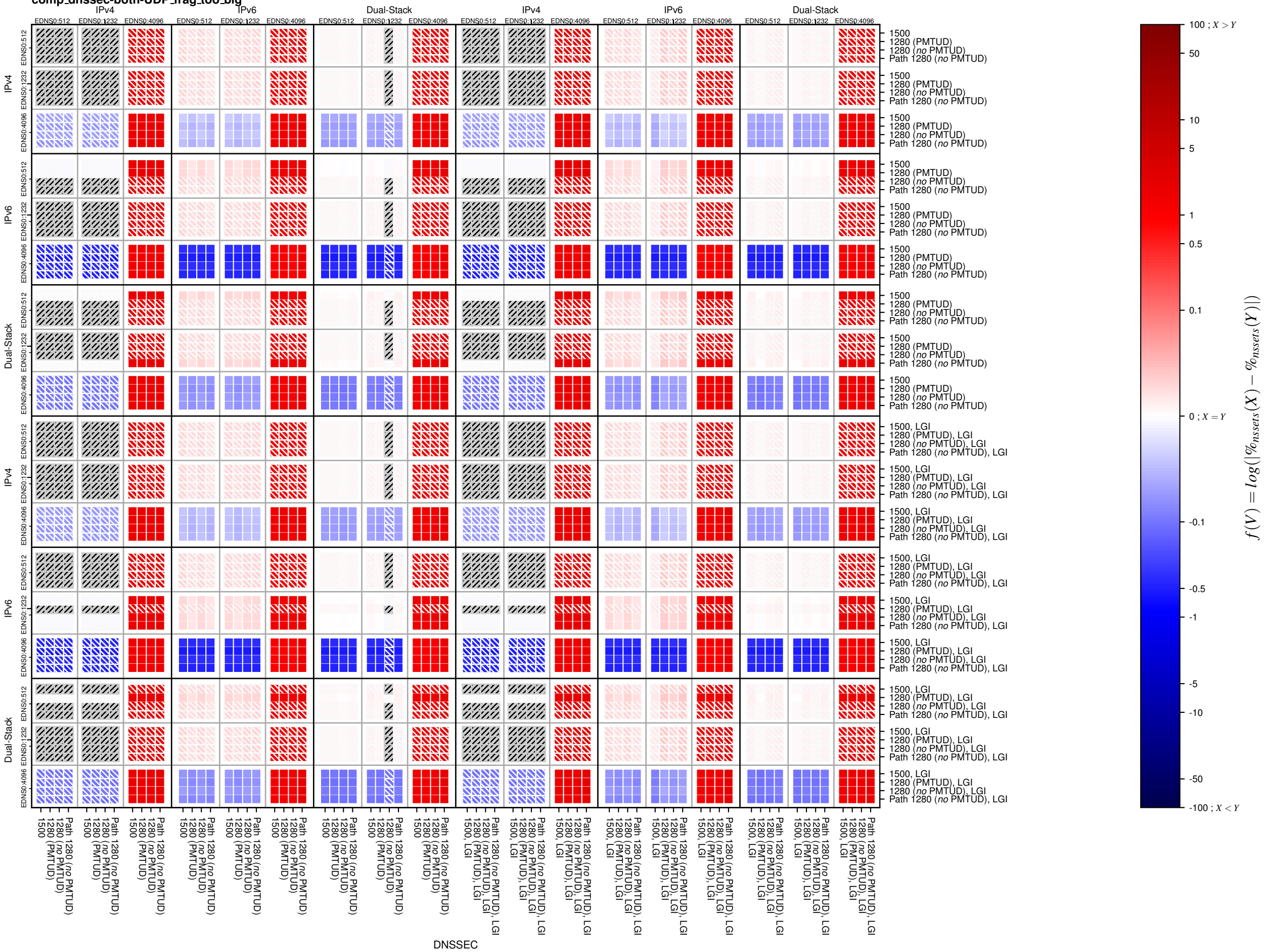
comp_dnssec-both-UDP_frag_too_big
