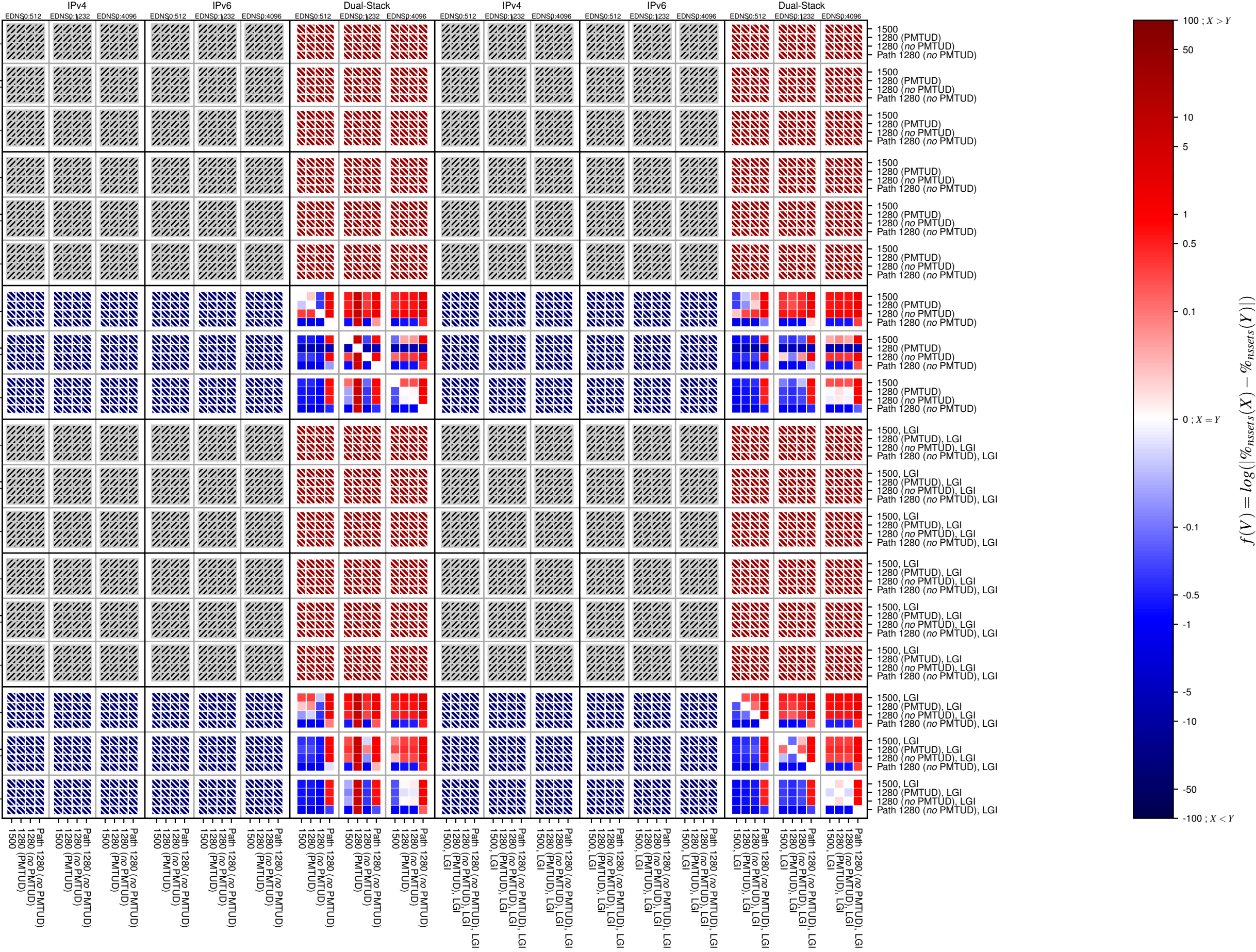
dnssec-v6-UDP_TCP_afi_count
